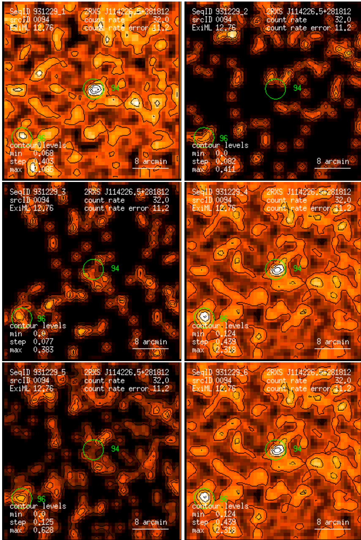
Figure 94: RASS 931229: detection 0094: band rate images, Gaussian filter: (1) PSPC channels 11 – 41, (2) 52 – 90, (3) 91 – 201, (4) 11 – 235, (5) 52 – 201, (6) 11 – 201. Broad band rates in counts/ks. Band rate contour levels in counts/ks/arcmin 2 .
