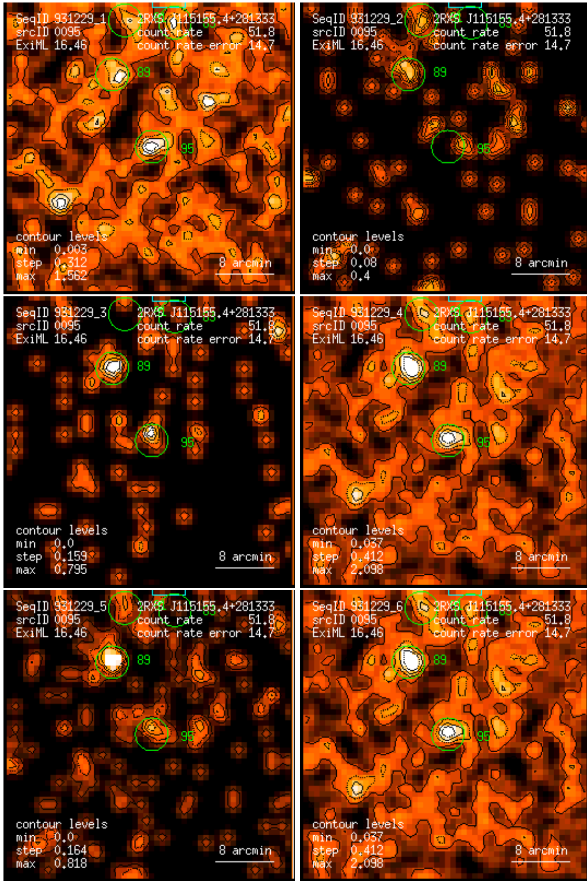
Figure 95: RASS 931229: detection 0095: band rate images, Gaussian filter: (1) PSPC channels 11 – 41, (2) 52 – 90, (3) 91 – 201, (4) 11 – 235, (5) 52 – 201, (6) 11 – 201. Broad band rates in counts/ks. Band rate contour levels in counts/ks/arcmin 2 .
