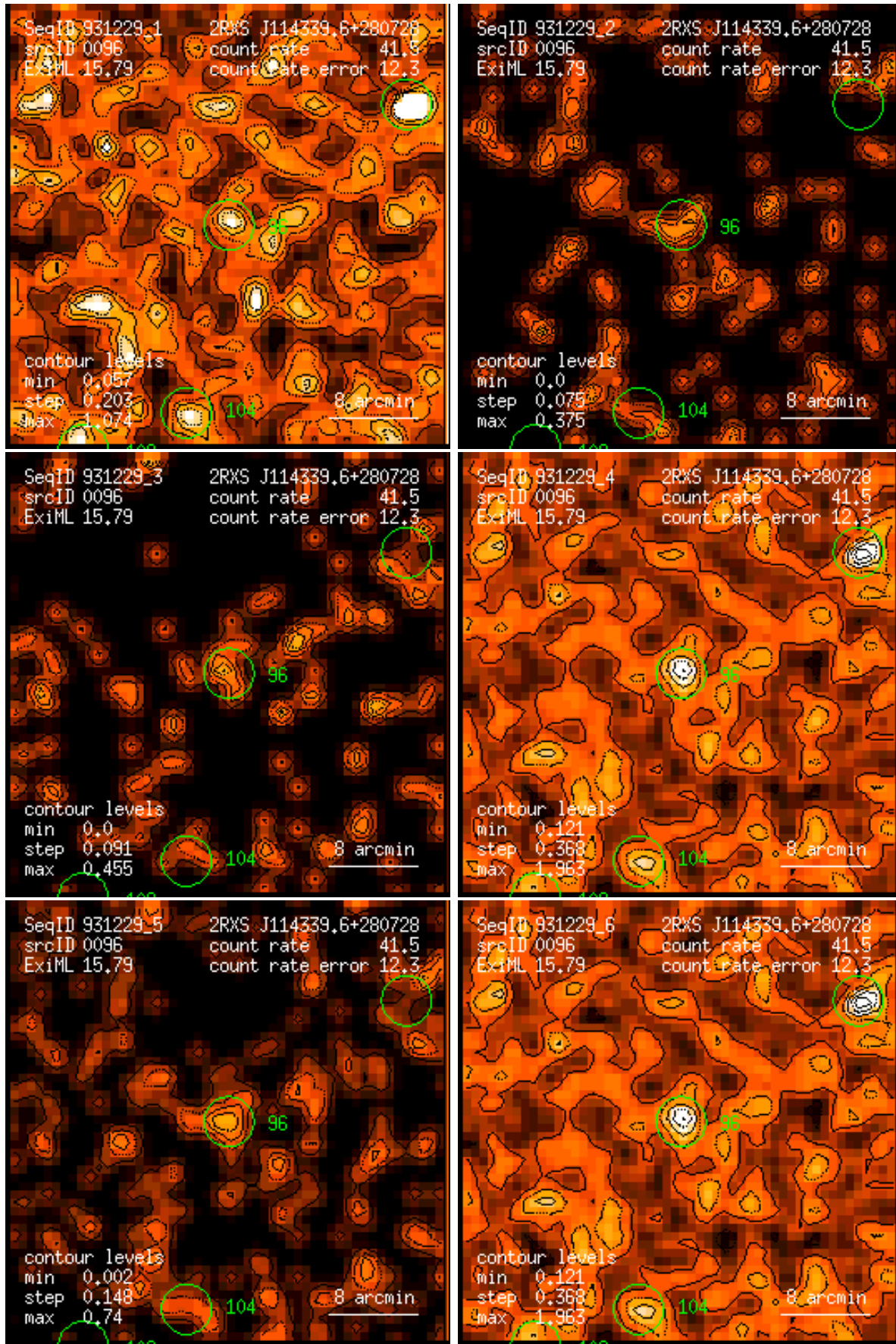
Figure 96: RASS 931229: detection 0096: band rate images, Gaussian filter: (1) PSPC channels 11 – 41, (2) 52 – 90, (3) 91 – 201, (4) 11 – 235, (5) 52 – 201, (6) 11 – 201. Broad band rates in counts/ks. Band rate contour levels in counts/ks/arcmin 2 .
