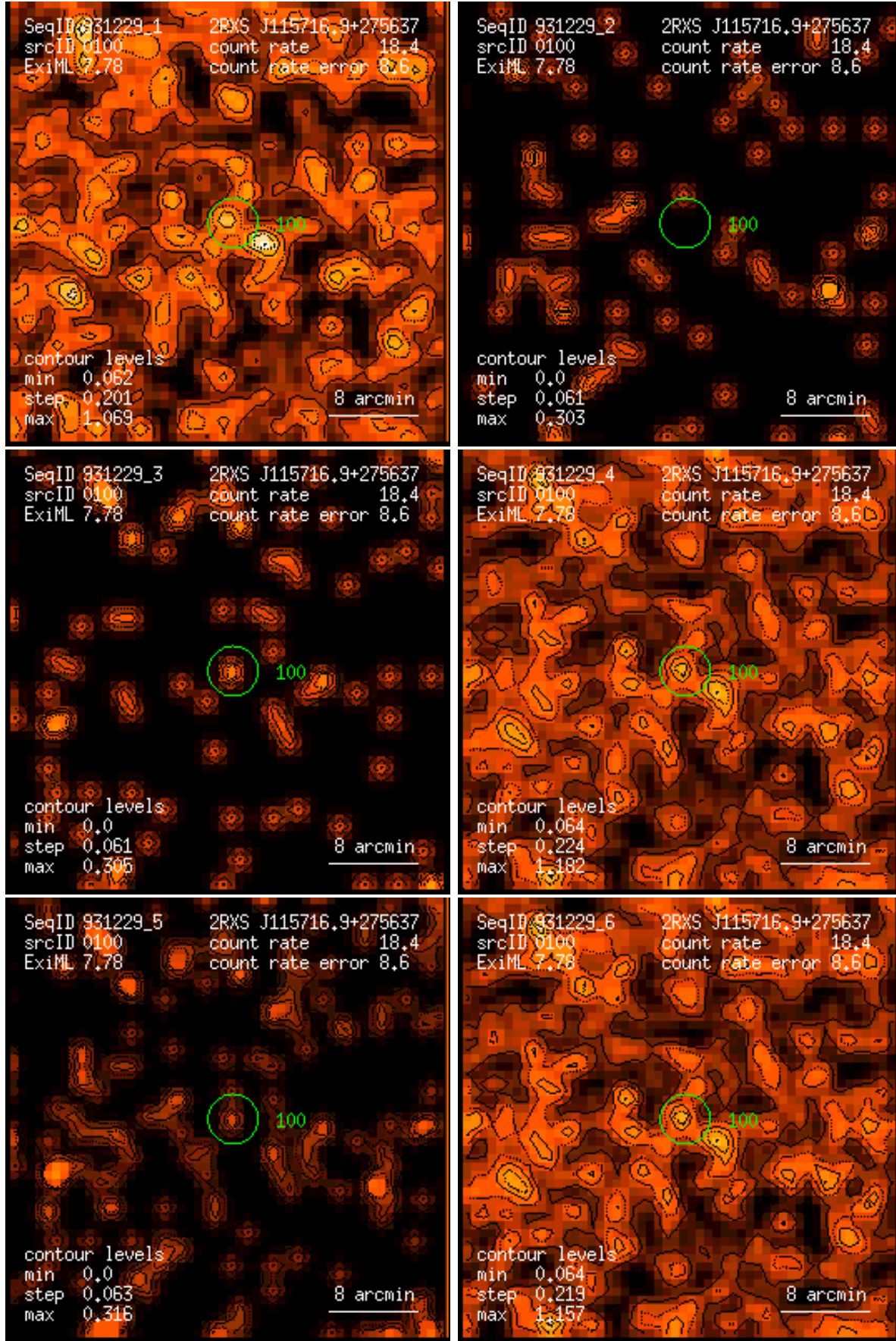
Figure 100: RASS 931229: detection 0100: band rate images, Gaussian filter: (1) PSPC channels 11 – 41, (2) 52 – 90, (3) 91 – 201, (4) 11 – 235, (5) 52 – 201, (6) 11 – 201. Broad band rates in counts/ks. Band rate contour levels in counts/ks/arcmin 2 .
