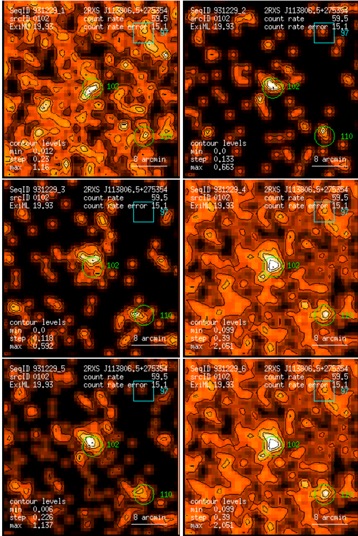
Figure 102: RASS 931229: detection 0102: band rate images, Gaussian filter: (1) PSPC channels 11 – 41, (2) 52 – 90, (3) 91 – 201, (4) 11 – 235, (5) 52 – 201, (6) 11 – 201. Broad band rates in counts/ks. Band rate contour levels in counts/ks/arcmin 2 .
