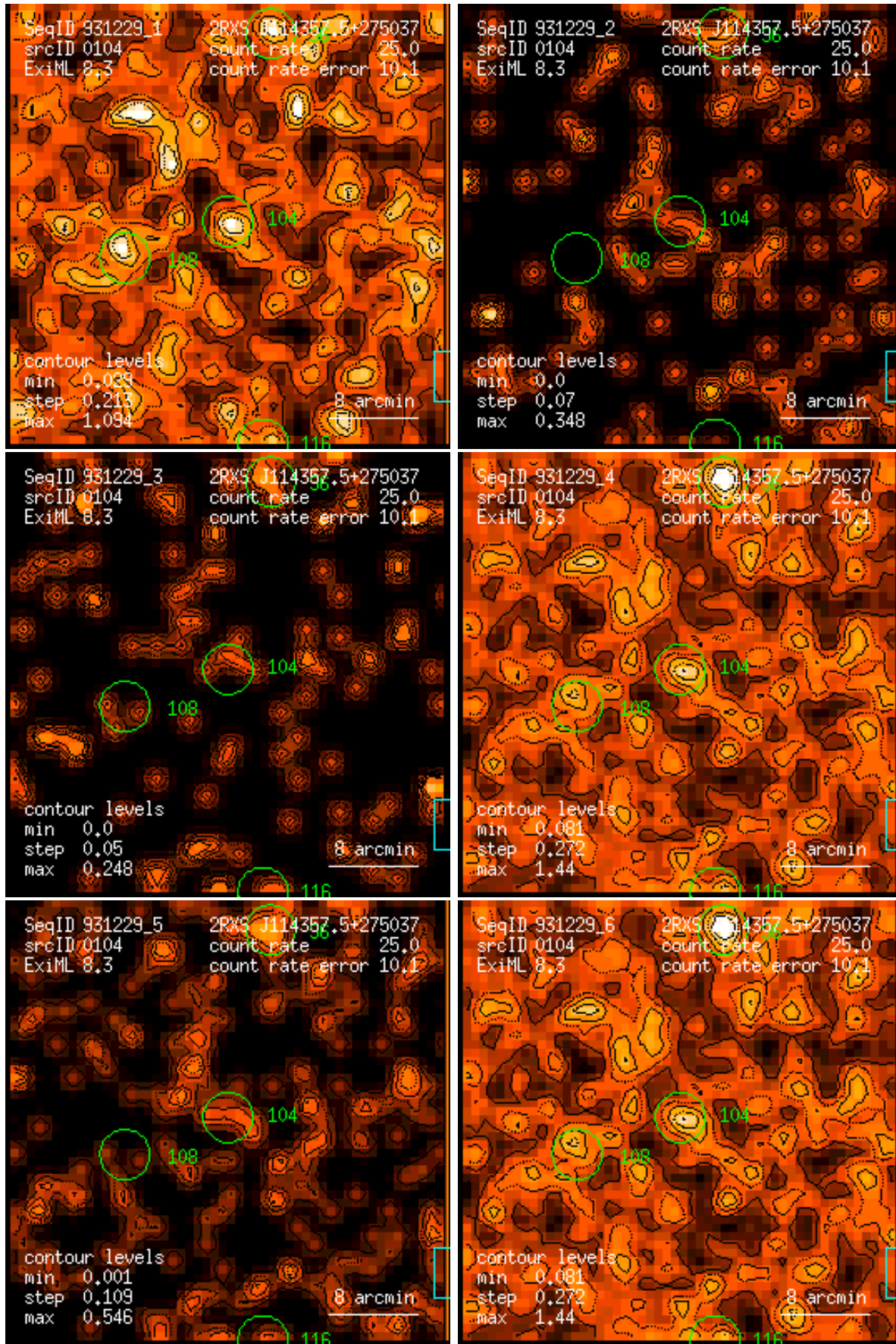
Figure 104: RASS 931229: detection 0104: band rate images, Gaussian filter: (1) PSPC channels 11 – 41, (2) 52 – 90, (3) 91 – 201, (4) 11 – 235, (5) 52 – 201, (6) 11 – 201. Broad band rates in counts/ks. Band rate contour levels in counts/ks/arcmin 2 .
