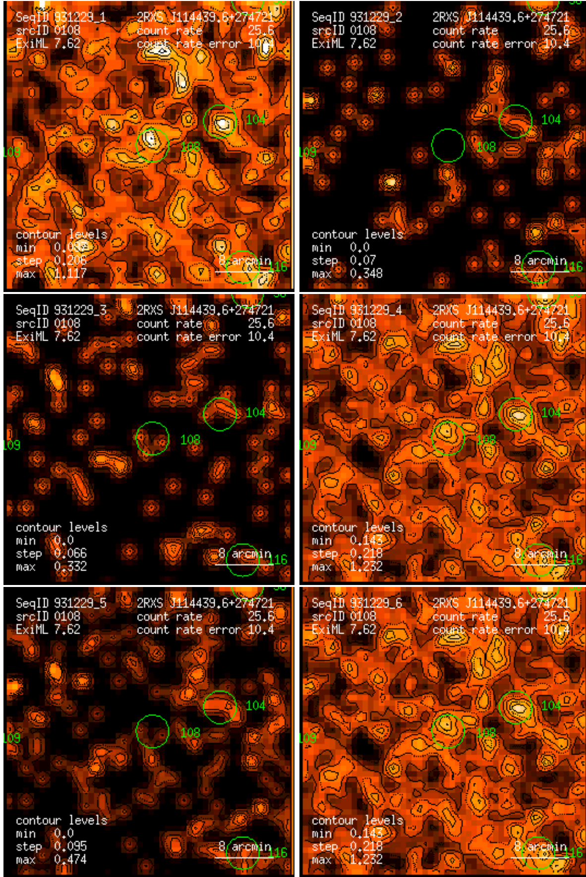
Figure 108: RASS 931229: detection 0108: band rate images, Gaussian filter: (1) PSPC channels 11 – 41, (2) 52 – 90, (3) 91 – 201, (4) 11 – 235, (5) 52 – 201, (6) 11 – 201. Broad band rates in counts/ks. Band rate contour levels in counts/ks/arcmin 2 .
