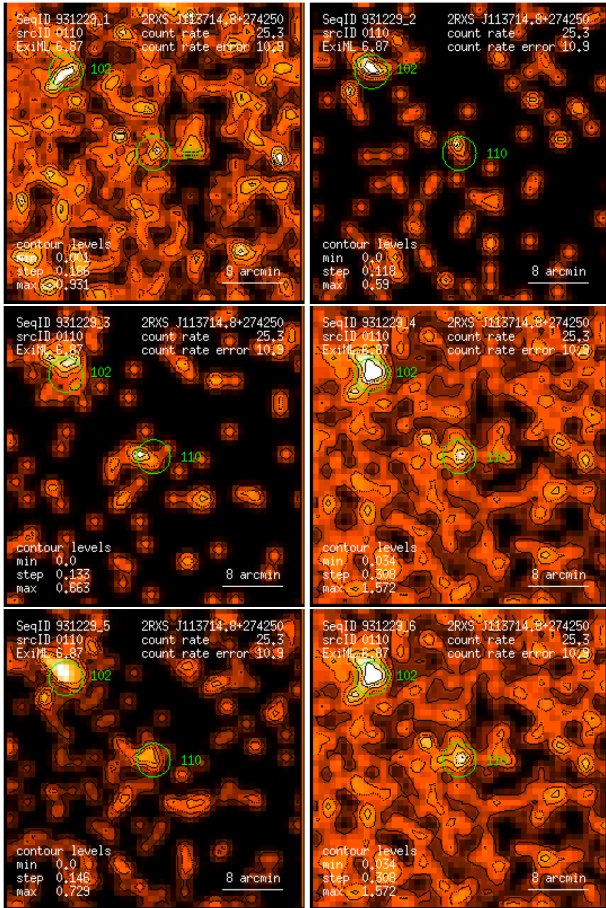
Figure 110: RASS 931229: detection 0110: band rate images, Gaussian filter: (1) PSPC channels 11 – 41, (2) 52 – 90, (3) 91 – 201, (4) 11 – 235, (5) 52 – 201, (6) 11 – 201. Broad band rates in counts/ks. Band rate contour levels in counts/ks/arcmin 2 .
