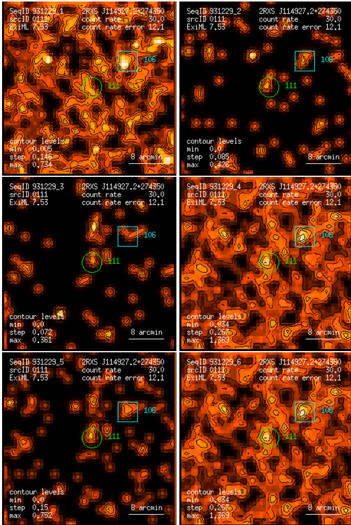
Figure 111: RASS 931229: detection 0111: band rate images, Gaussian filter: (1) PSPP channels 11 – 41, (2) 52 – 90, (3) 91 – 201, (4) 11 – 235, (5) 52 – 201, (6) 11 – 201. Broad band rates in counts/ks. Band rate contour levels in counts/ks/arcmin 2 .
