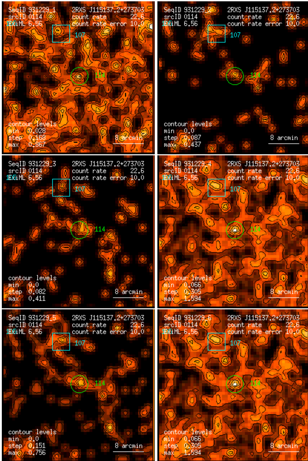
Figure 114: RASS 931229: detection 0114: band rate images, Gaussian filter: (1) PSPC channels 11 – 41, (2) 52 – 90, (3) 91 – 201, (4) 11 – 235, (5) 52 – 201, (6) 11 – 201. Broad band rates in counts/ks. Band rate contour levels in counts/ks/arcmin 2 .
