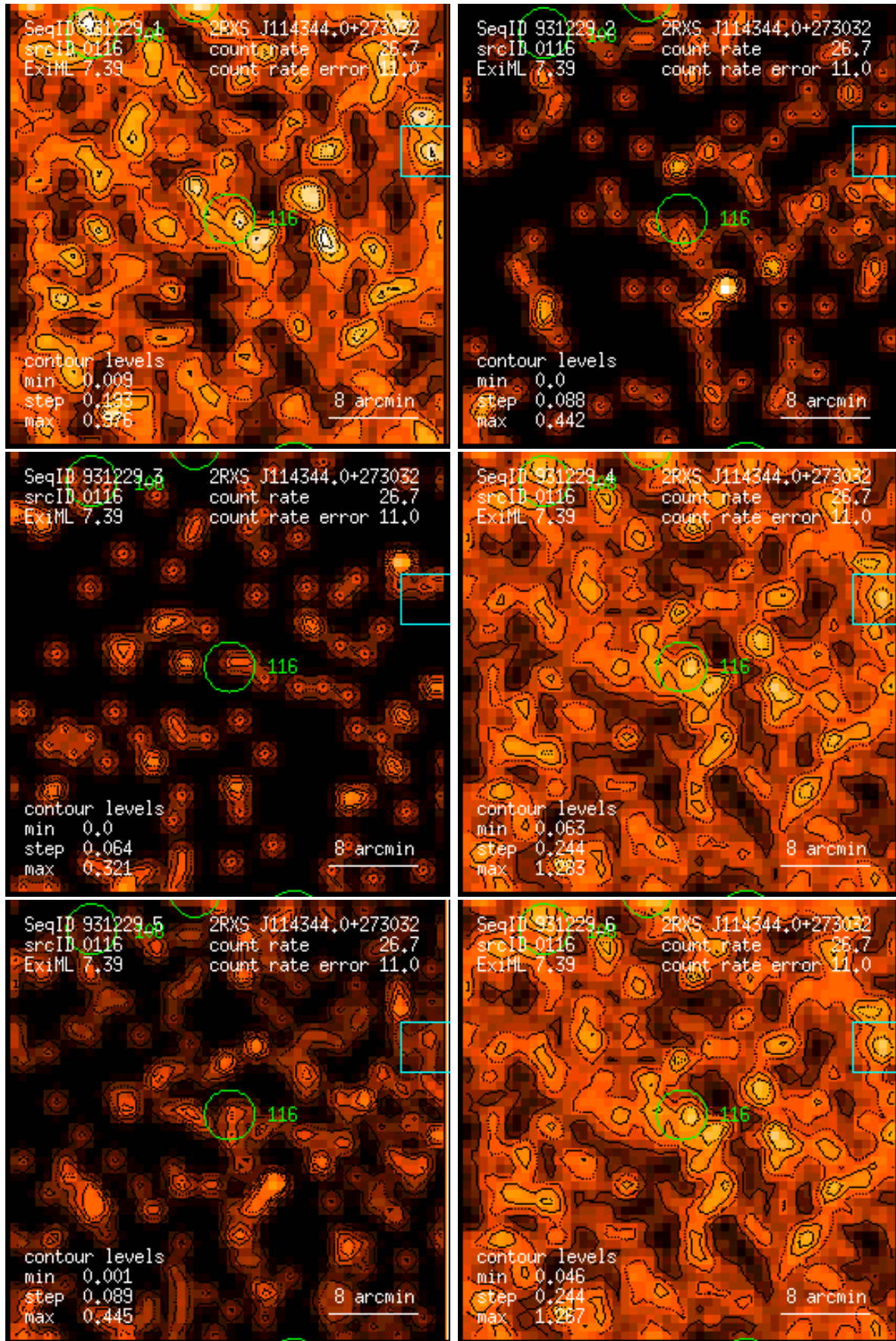
Figure 116: RASS 931229: detection 0116: band rate images, Gaussian filter: (1) PSPC channels 11 – 41, (2) 52 – 90, (3) 91 – 201, (4) 11 – 235, (5) 52 – 201, (6) 11 – 201. Broad band rates in counts/ks. Band rate contour levels in counts/ks/arcmin 2 .
