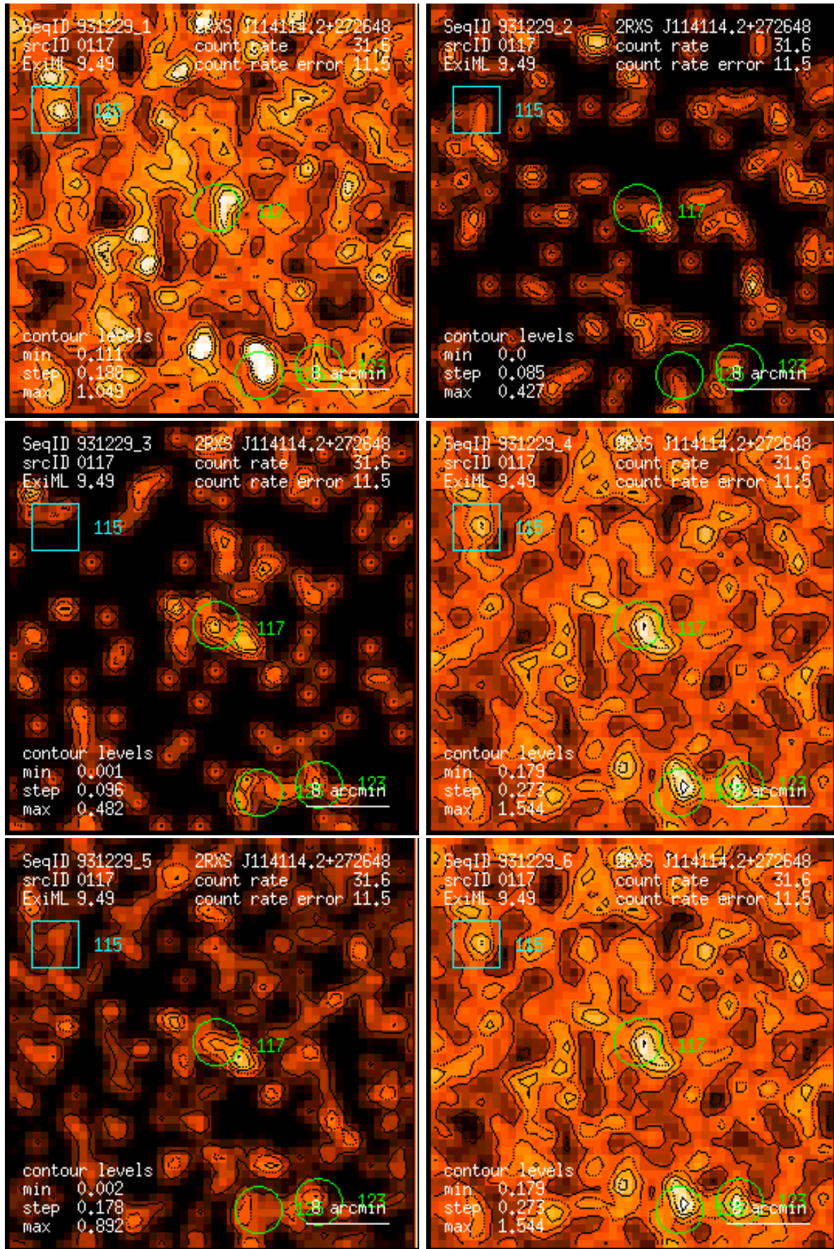
Figure 117: RASS 931229: detection 0117: band rate images, Gaussian filter: (1) PSPC channels 11 – 41, (2) 52 – 90, (3) 91 – 201, (4) 11 – 235, (5) 52 – 201, (6) 11 – 201. Broad band rates in counts/ks. Band rate contour levels in counts/ks/arcmin 2 .
