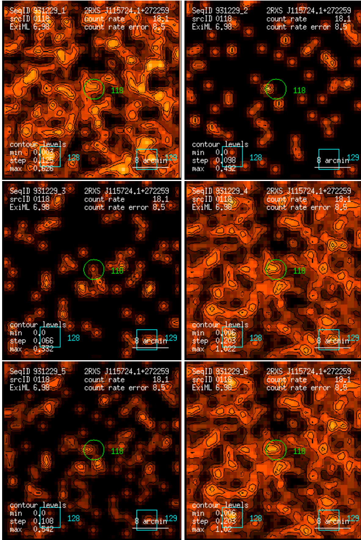
Figure 118: RASS 931229: detection 0118: band rate images, Gaussian filter: (1) PSPC channels 11 – 41, (2) 52 – 90, (3) 91 – 201, (4) 11 – 235, (5) 52 – 201, (6) 11 – 201. Broad band rates in counts/ks. Band rate contour levels in counts/ks/arcmin 2 .
