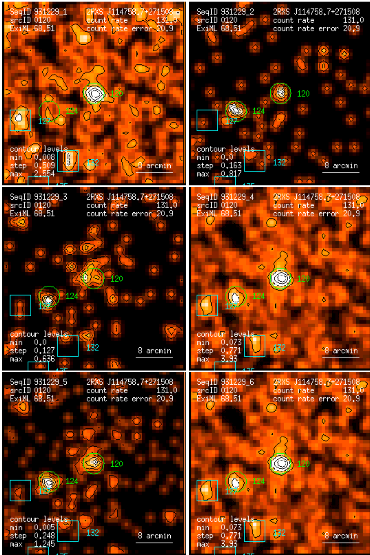
Figure 120: RASS 931229: detection 0120: band rate images, Gaussian filter: (1) PSPC channels 11 – 41, (2) 52 – 90, (3) 91 – 201, (4) 11 – 235, (5) 52 – 201, (6) 11 – 201. Broad band rates in counts/ks. Band rate contour levels in counts/ks/arcmin 2 .
