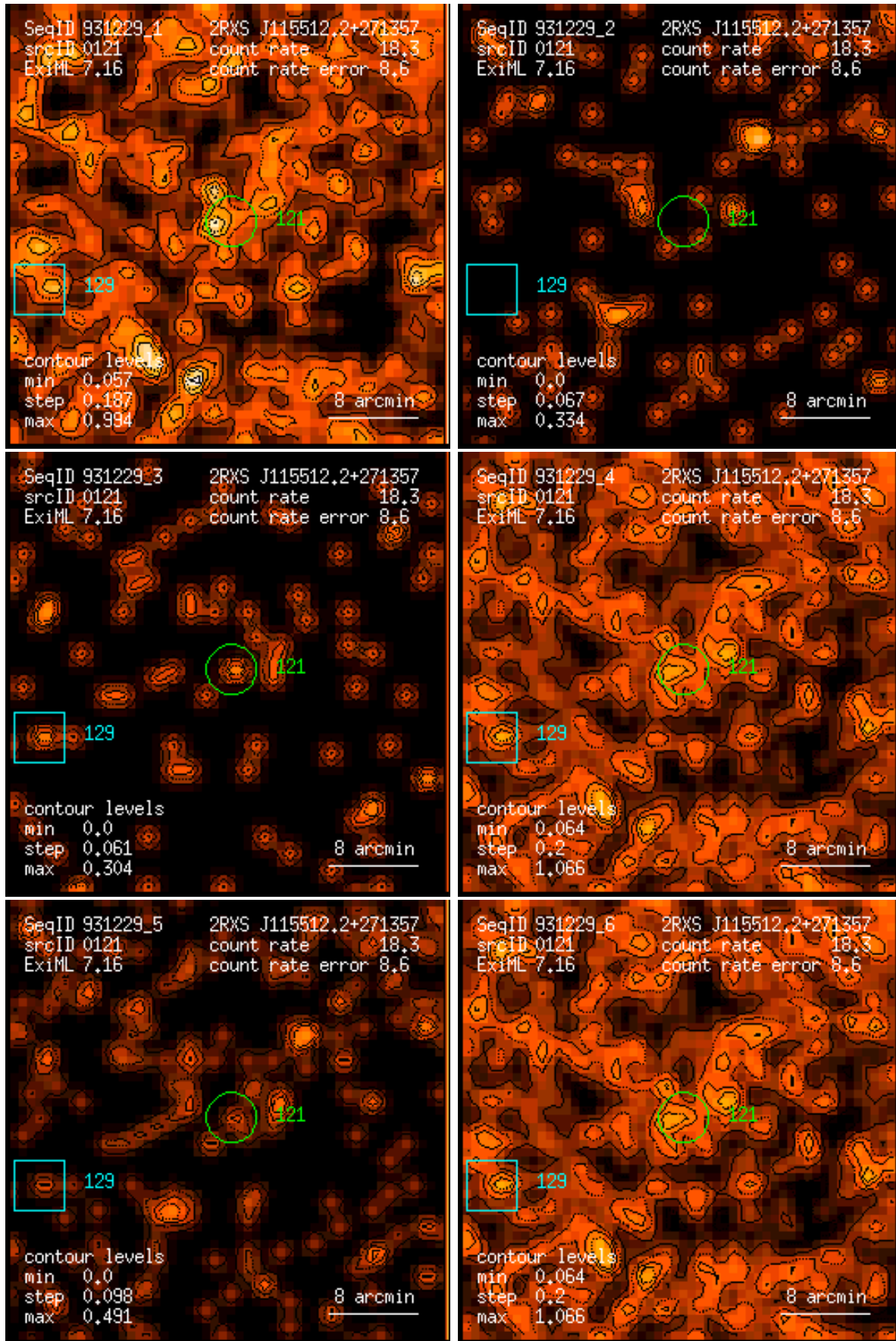
Figure 121: RASS 931229: detection 0121: band rate images, Gaussian filter: (1) PSPC channels 11 – 41, (2) 52 – 90, (3) 91 – 201, (4) 11 – 235, (5) 52 – 201, (6) 11 – 201. Broad band rates in counts/ks. Band rate contour levels in counts/ks/arcmin 2 .
