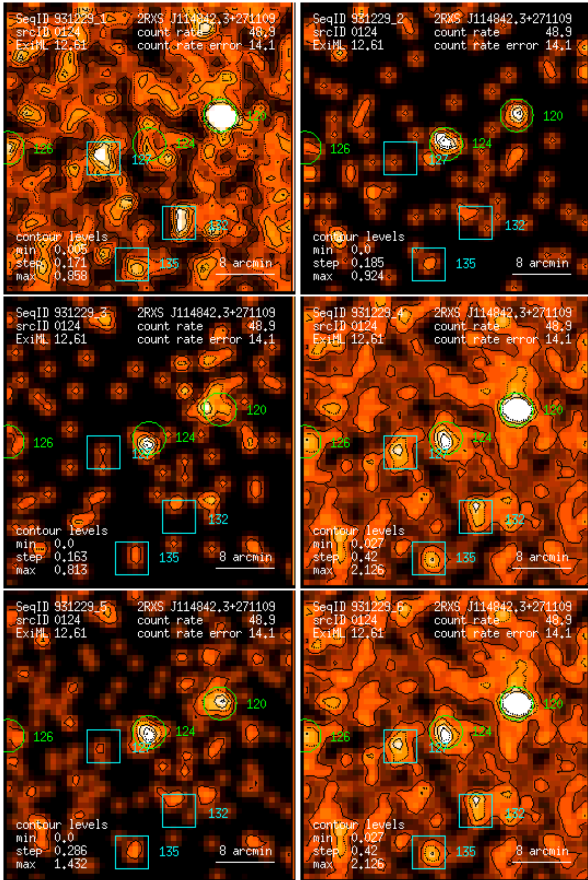
Figure 124: RASS 931229: detection 0124: band rate images, Gaussian filter: (1) PSPC channels 11 – 41, (2) 52 – 90, (3) 91 – 201, (4) 11 – 235, (5) 52 – 201, (6) 11 – 201. Broad band rates in counts/ks. Band rate contour levels in counts/ks/arcmin 2 .
