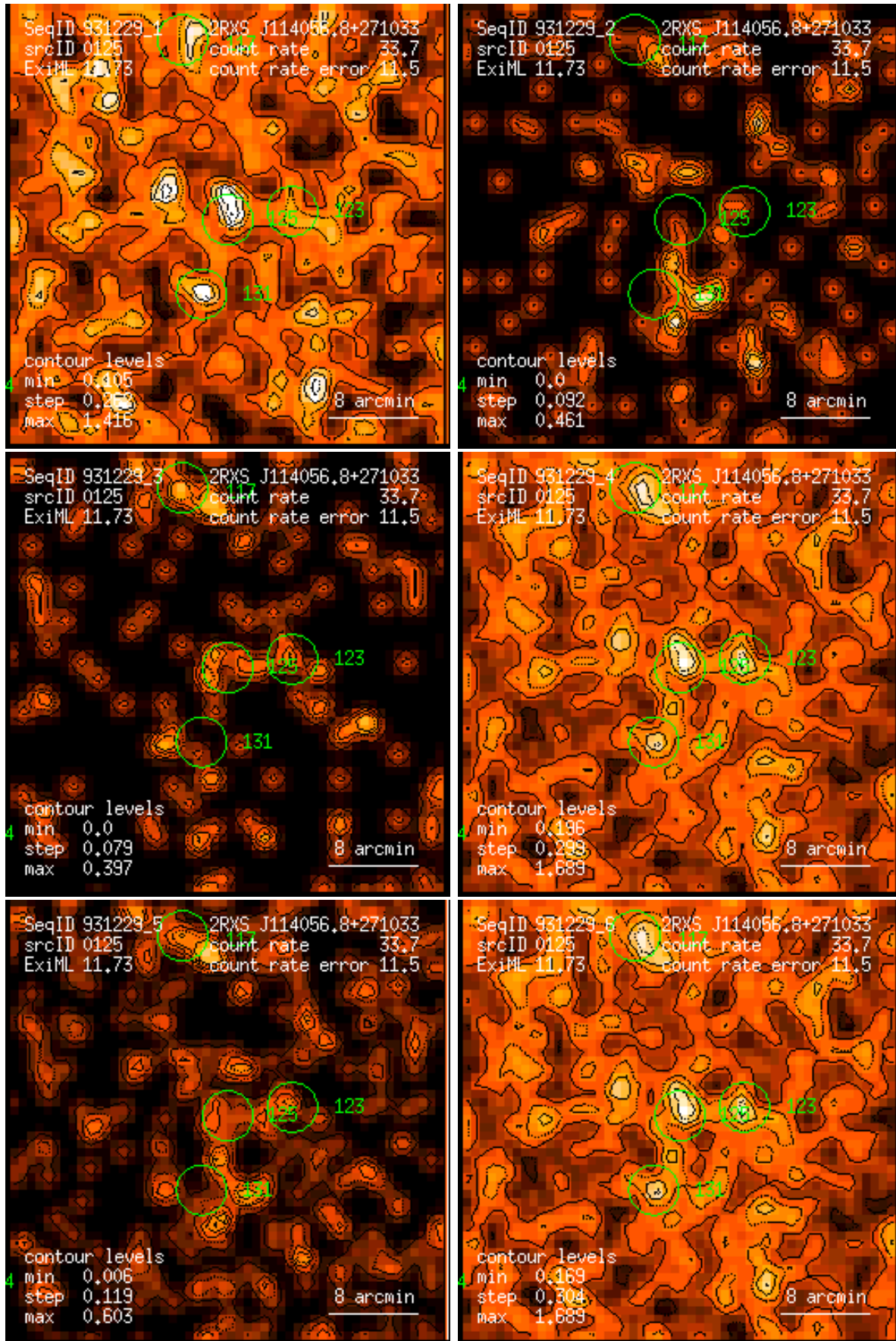
Figure 125: RASS 931229: detection 0125: band rate images, Gaussian filter: (1) PSPC channels 11 – 41, (2) 52 – 90, (3) 91 – 201, (4) 11 – 235, (5) 52 – 201, (6) 11 – 201. Broad band rates in counts/ks. Band rate contour levels in counts/ks/arcmin 2 .
