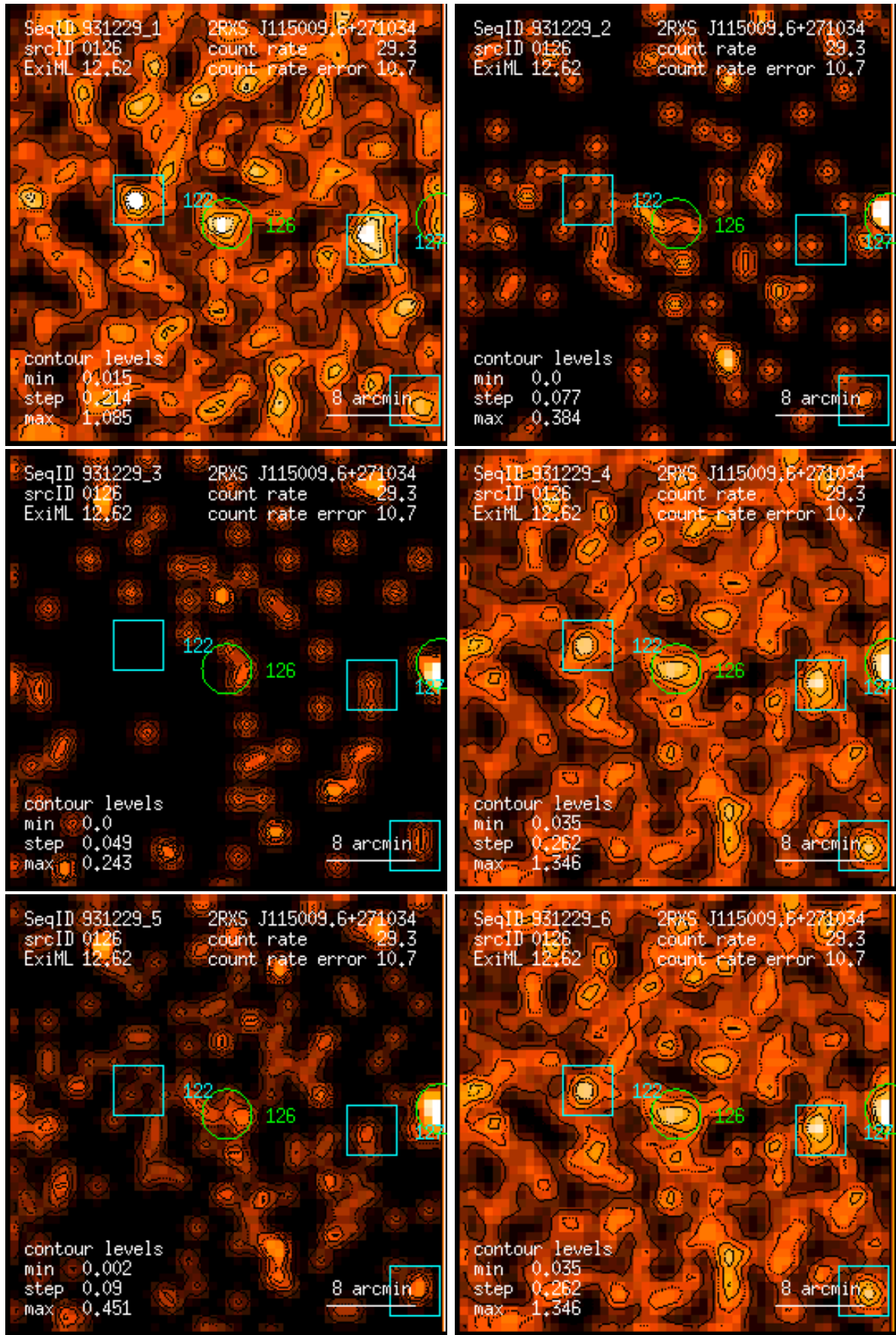
Figure 126: RASS 931229: detection 0126: band rate images, Gaussian filter: (1) PSPC channels 11 – 41, (2) 52 – 90, (3) 91 – 201, (4) 11 – 235, (5) 52 – 201, (6) 11 – 201. Broad band rates in counts/ks. Band rate contour levels in counts/ks/arcmin 2 .
