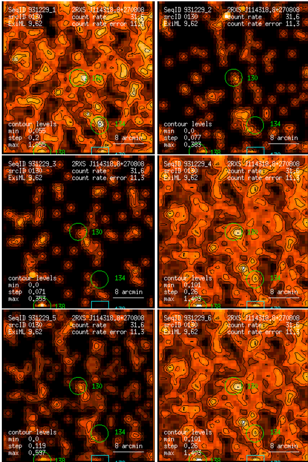
Figure 130: RASS 931229: detection 0130: band rate images, Gaussian filter: (1) PSPC channels 11 – 41, (2) 52 – 90, (3) 91 – 201, (4) 11 – 235, (5) 52 – 201, (6) 11 – 201. Broad band rates in counts/ks. Band rate contour levels in counts/ks/arcmin 2 .
