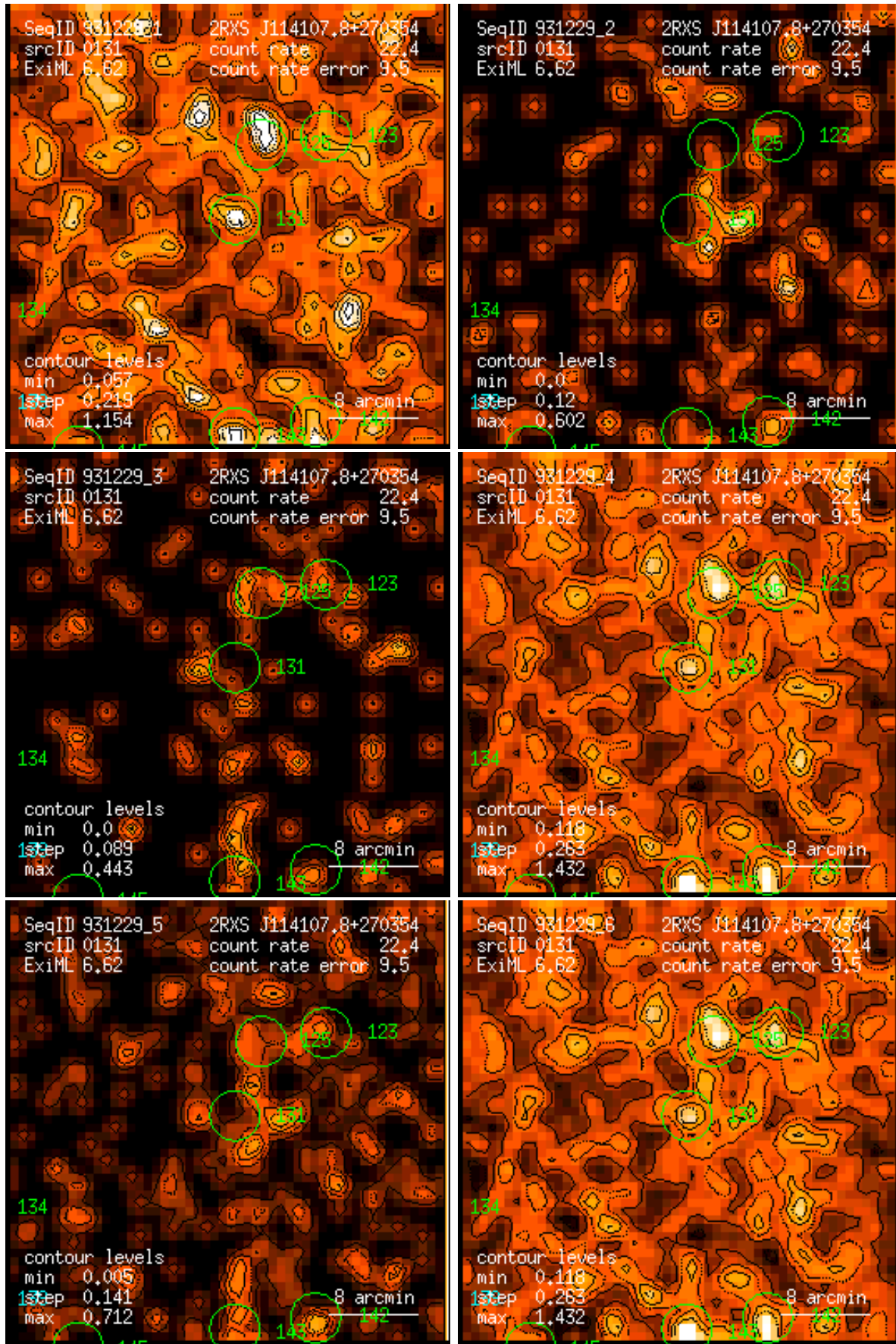
Figure 131: RASS 931229: detection 0131: band rate images, Gaussian filter: (1) PSPC channels 11 – 41, (2) 52 – 90, (3) 91 – 201, (4) 11 – 235, (5) 52 – 201, (6) 11 – 201. Broad band rates in counts/ks. Band rate contour levels in counts/ks/arcmin 2 .
