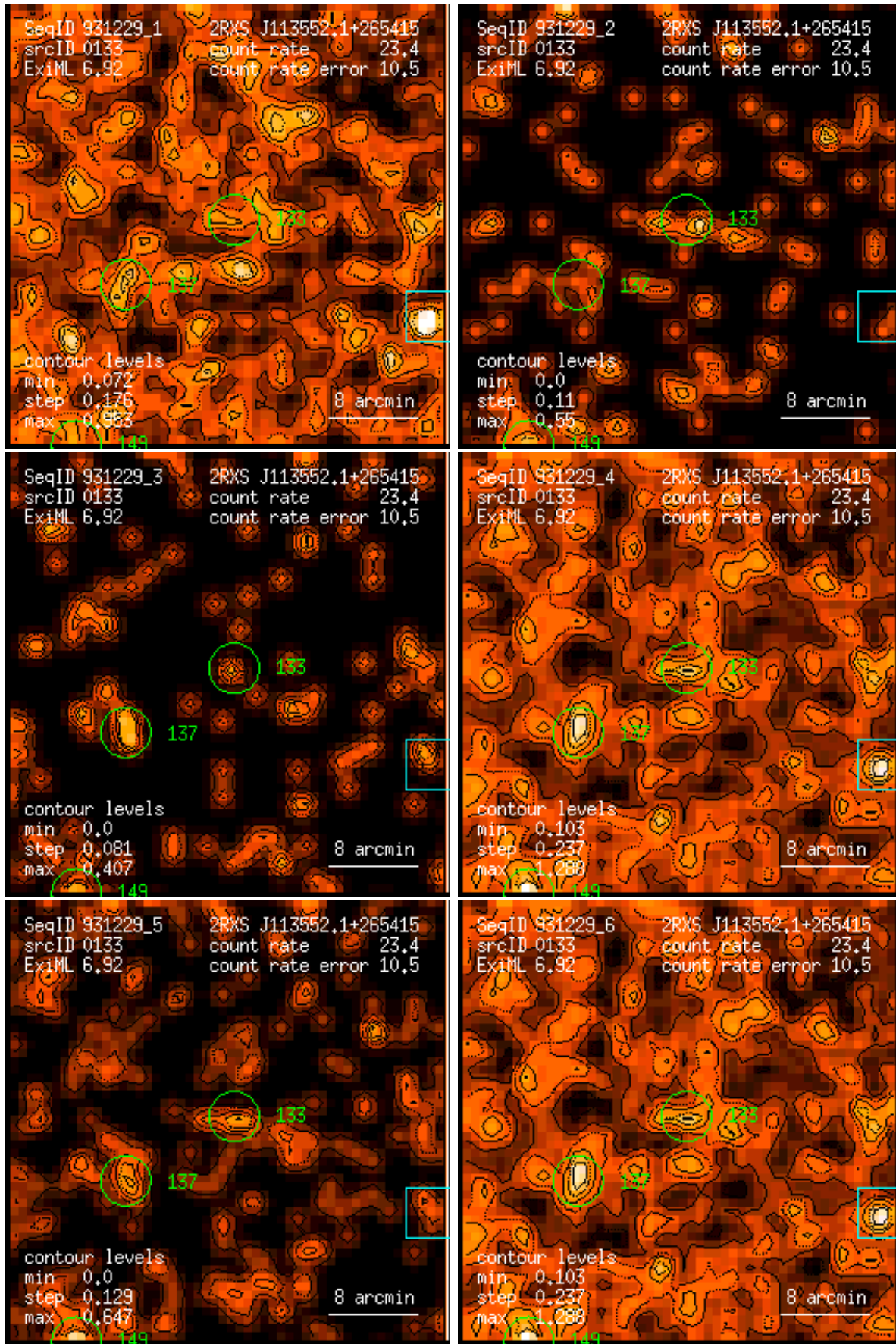
Figure 133: RASS 931229: detection 0133: band rate images, Gaussian filter: (1) PSPC channels 11 – 41, (2) 52 – 90, (3) 91 – 201, (4) 11 – 235, (5) 52 – 201, (6) 11 – 201. Broad band rates in counts/ks. Band rate contour levels in counts/ks/arcmin 2 .
