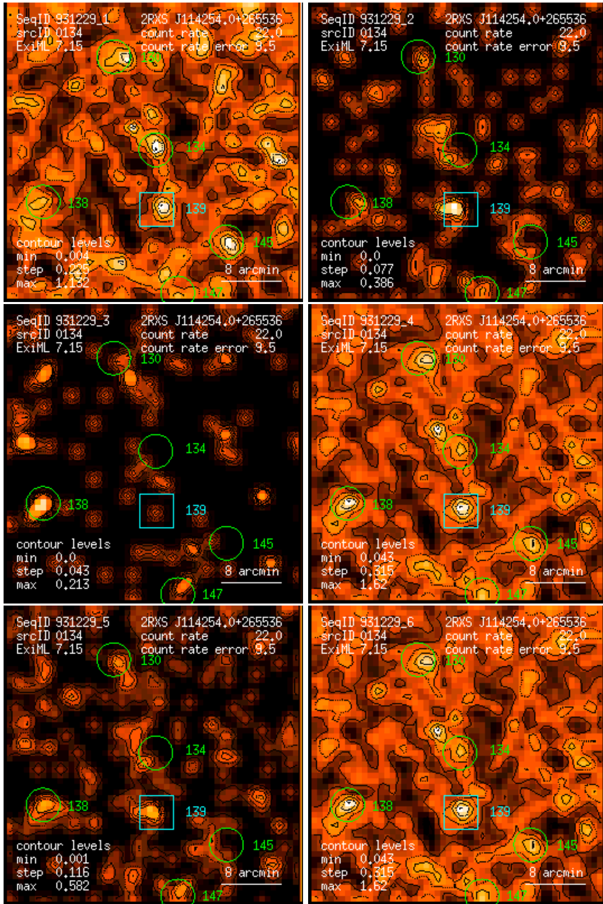
Figure 134: RASS 931229: detection 0134: band rate images, Gaussian filter: (1) PSPC channels 11 – 41, (2) 52 – 90, (3) 91 – 201, (4) 11 – 235, (5) 52 – 201, (6) 11 – 201. Broad band rates in counts/ks. Band rate contour levels in counts/ks/arcmin 2 .
