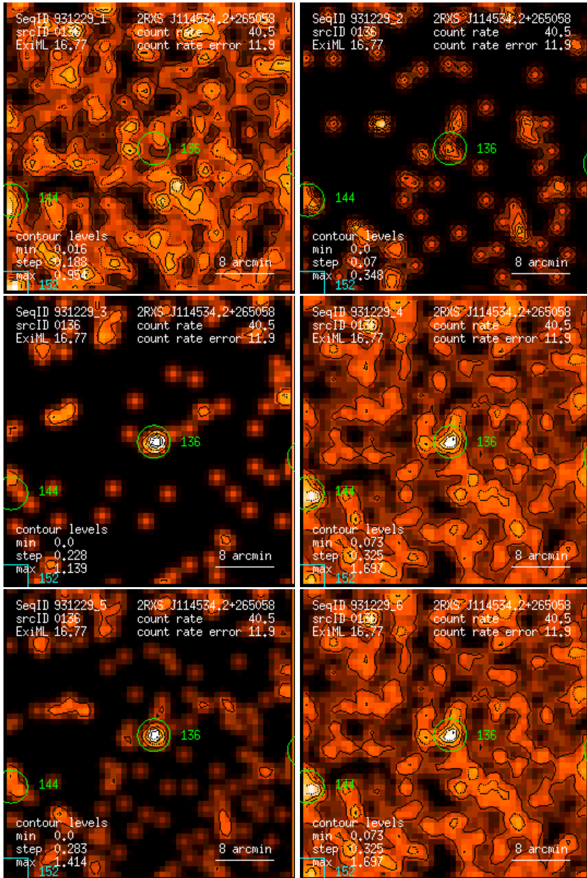
Figure 136: RASS 931229: detection 0136: band rate images, Gaussian filter: (1) PSPC channels 11 – 41, (2) 52 – 90, (3) 91 – 201, (4) 11 – 235, (5) 52 – 201, (6) 11 – 201. Broad band rates in counts/ks. Band rate contour levels in counts/ks/arcmin 2 .
