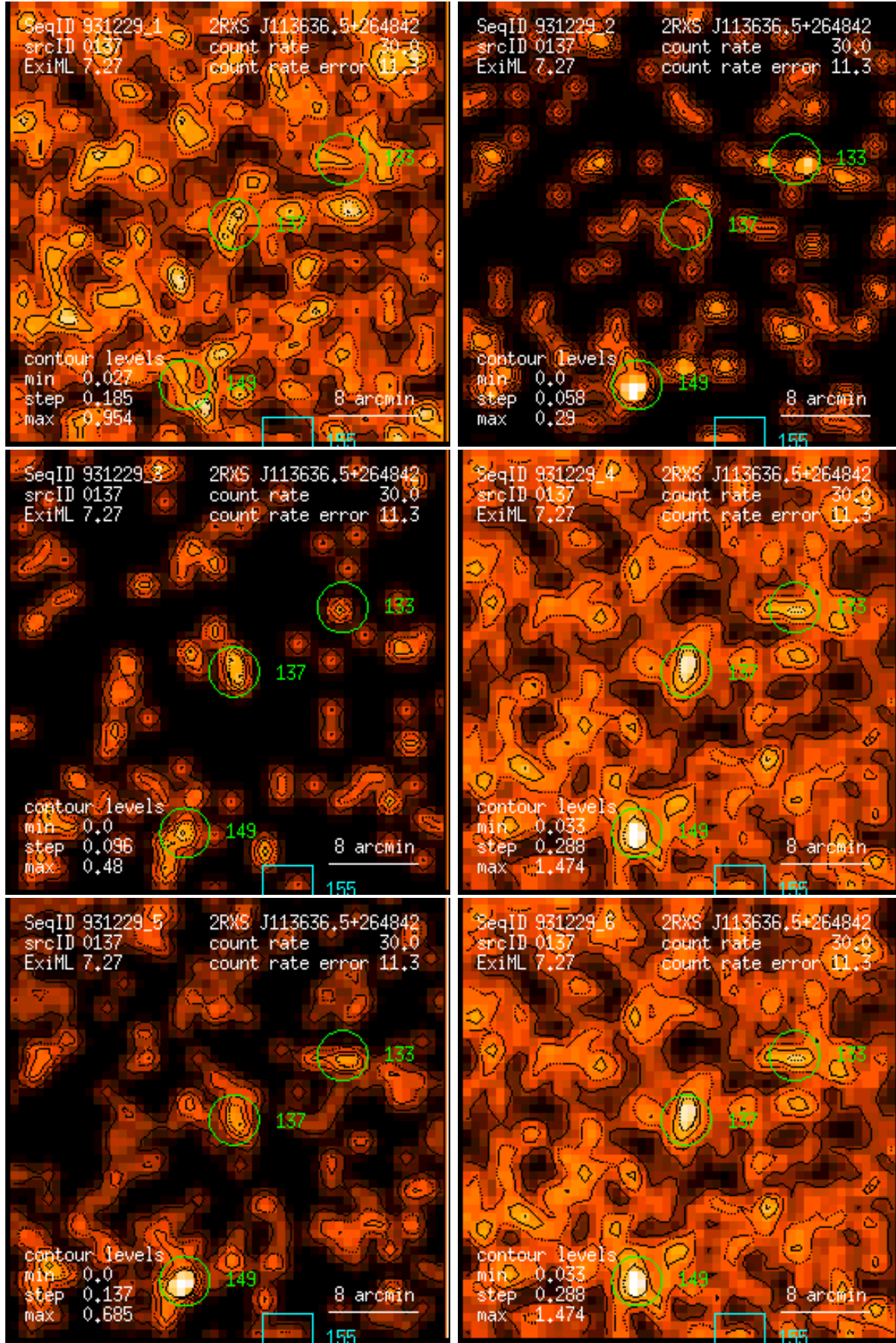
Figure 137: RASS 931229: detection 0137: band rate images, Gaussian filter: (1) PSPC channels 11 – 41, (2) 52 – 90, (3) 91 – 201, (4) 11 – 235, (5) 52 – 201, (6) 11 – 201. Broad band rates in counts/ks. Band rate contour levels in counts/ks/arcmin 2 .
