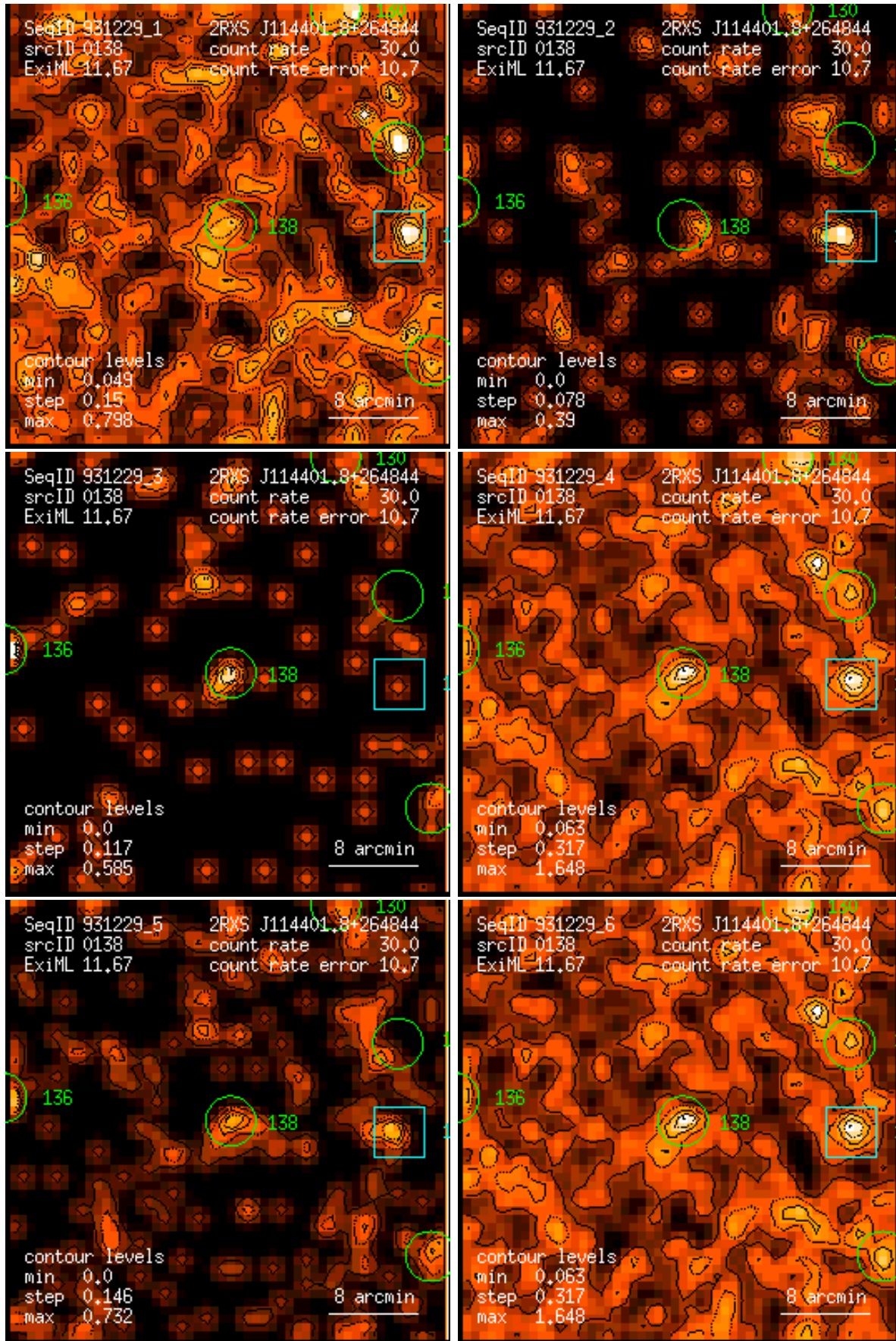
Figure 138: RASS 931229: detection 0138: band rate images, Gaussian filter: (1) PSPC channels 11 – 41, (2) 52 – 90, (3) 91 – 201, (4) 11 – 235, (5) 52 – 201, (6) 11 – 201. Broad band rates in counts/ks. Band rate contour levels in counts/ks/arcmin 2 .
