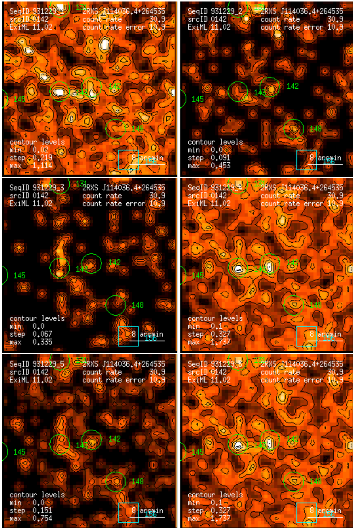
Figure 142: RASS 931229: detection 0142: band rate images, Gaussian filter: (1) PSPC channels 11 – 41, (2) 52 – 90, (3) 91 – 201, (4) 11 – 235, (5) 52 – 201, (6) 11 – 201. Broad band rates in counts/ks. Band rate contour levels in counts/ks/arcmin 2 .
