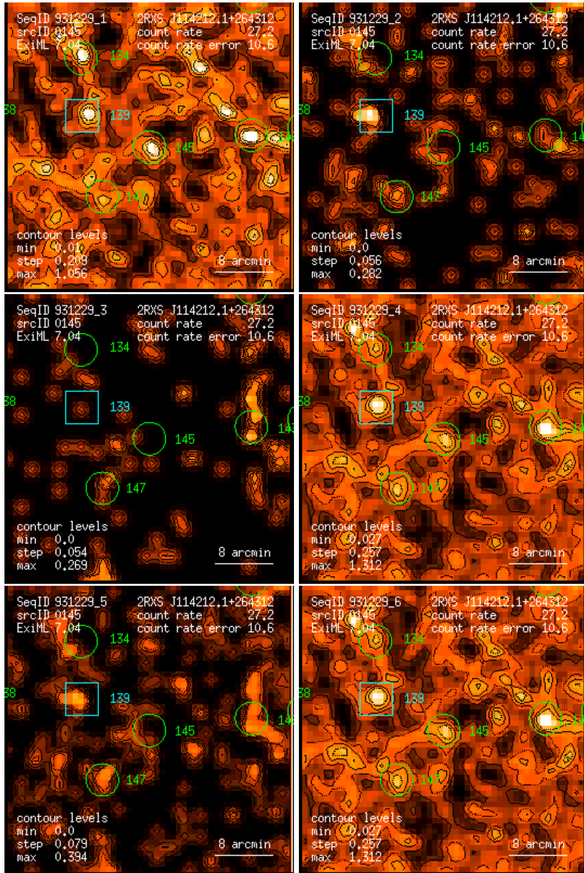
Figure 145: RASS 931229: detection 0145: band rate images, Gaussian filter: (1) PSPC channels 11 – 41, (2) 52 – 90, (3) 91 – 201, (4) 11 – 235, (5) 52 – 201, (6) 11 – 201. Broad band rates in counts/ks. Band rate contour levels in counts/ks/arcmin 2 .
