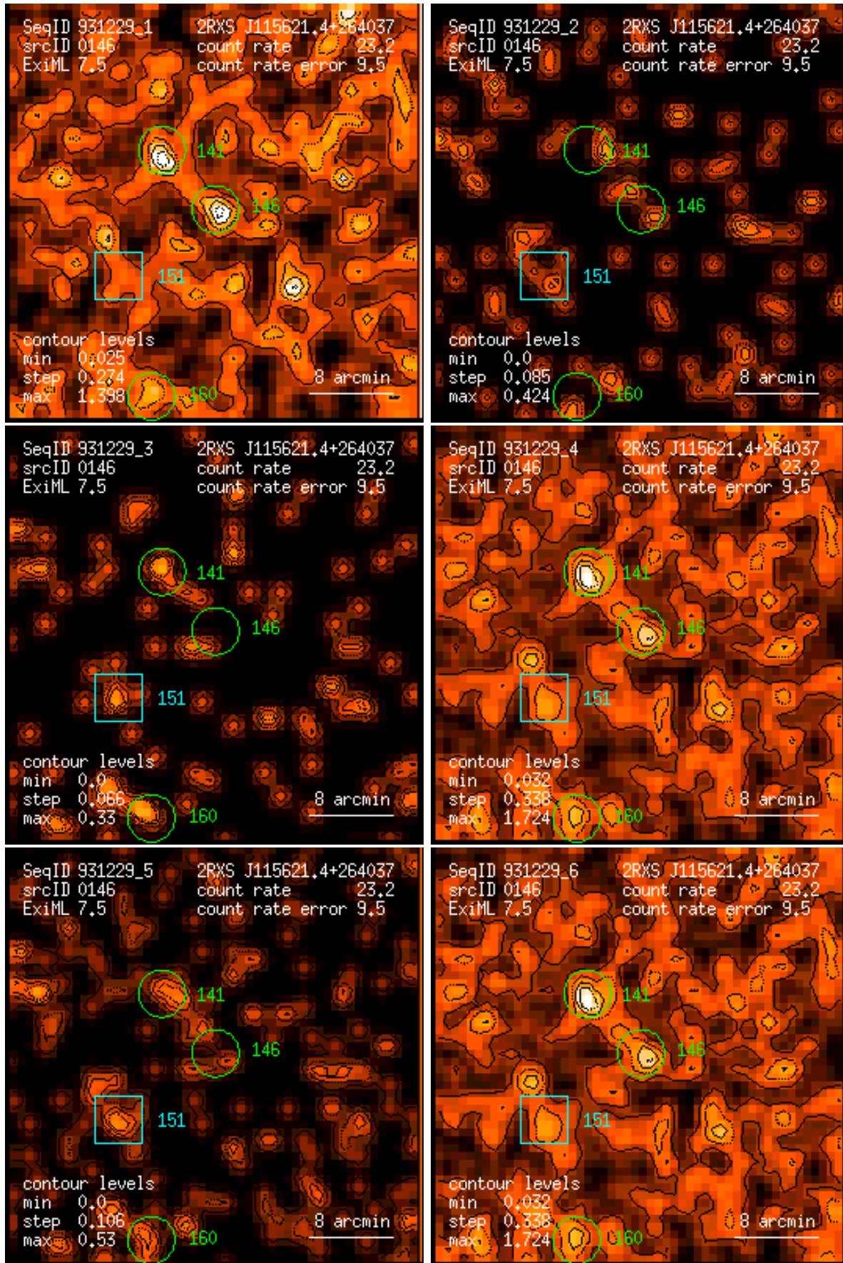
Figure 146: RASS 931229: detection 0146: band rate images, Gaussian filter: (1) PSPC channels 11 – 41, (2) 52 – 90, (3) 91 – 201, (4) 11 – 235, (5) 52 – 201, (6) 11 – 201. Broad band rates in counts/ks. Band rate contour levels in counts/ks/arcmin 2 .
