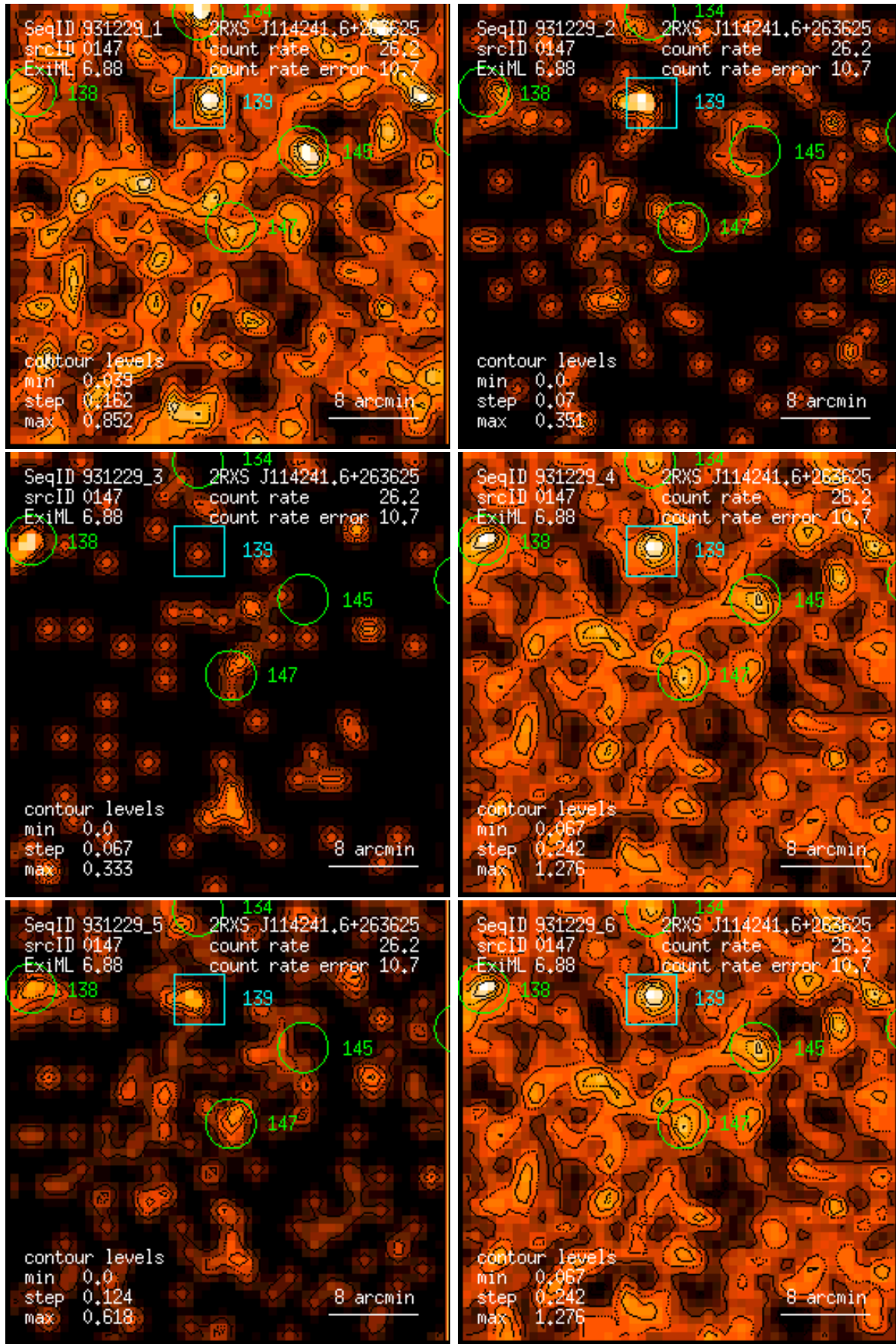
Figure 147: RASS 931229: detection 0147: band rate images, Gaussian filter: (1) PSPC channels 11 – 41, (2) 52 – 90, (3) 91 – 201, (4) 11 – 235, (5) 52 – 201, (6) 11 – 201. Broad band rates in counts/ks. Band rate contour levels in counts/ks/arcmin 2 .
