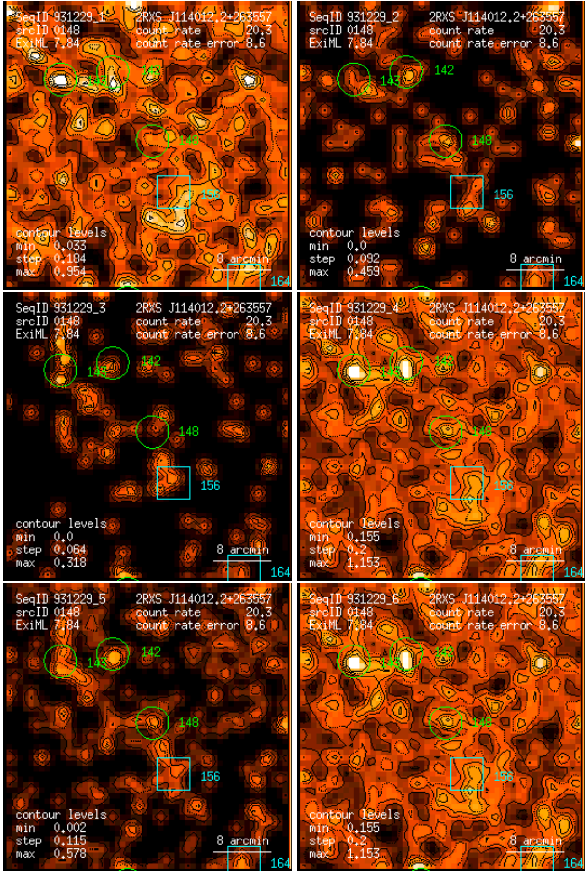
Figure 148: RASS 931229: detection 0148: band rate images, Gaussian filter: (1) PSPC channels 11 – 41, (2) 52 – 90, (3) 91 – 201, (4) 11 – 235, (5) 52 – 201, (6) 11 – 201. Broad band rates in counts/ks. Band rate contour levels in counts/ks/arcmin 2 .
