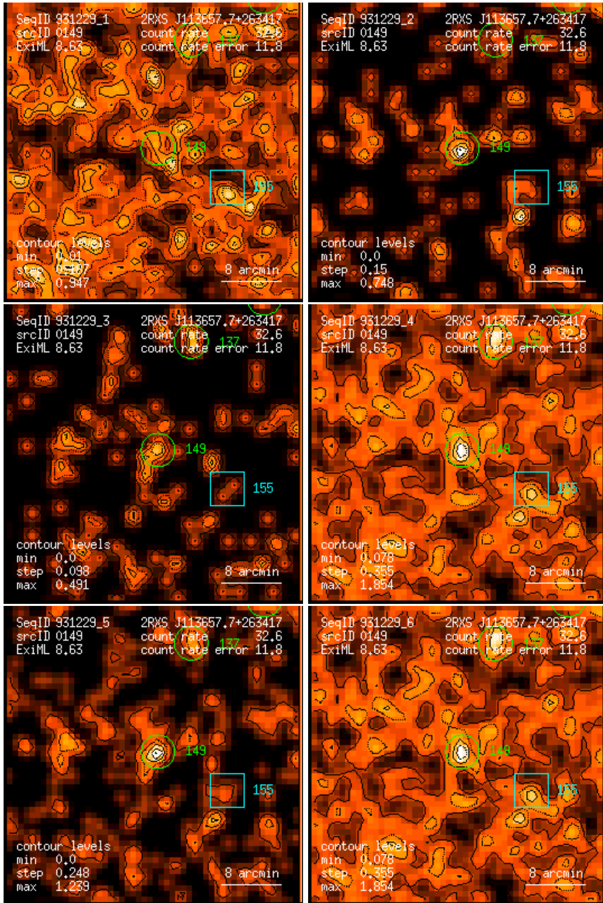
Figure 149: RASS 931229: detection 0149: band rate images, Gaussian filter: (1) PSPC channels 11 – 41, (2) 52 – 90, (3) 91 – 201, (4) 11 – 235, (5) 52 – 201, (6) 11 – 201. Broad band rates in counts/ks. Band rate contour levels in counts/ks/arcmin 2 .
