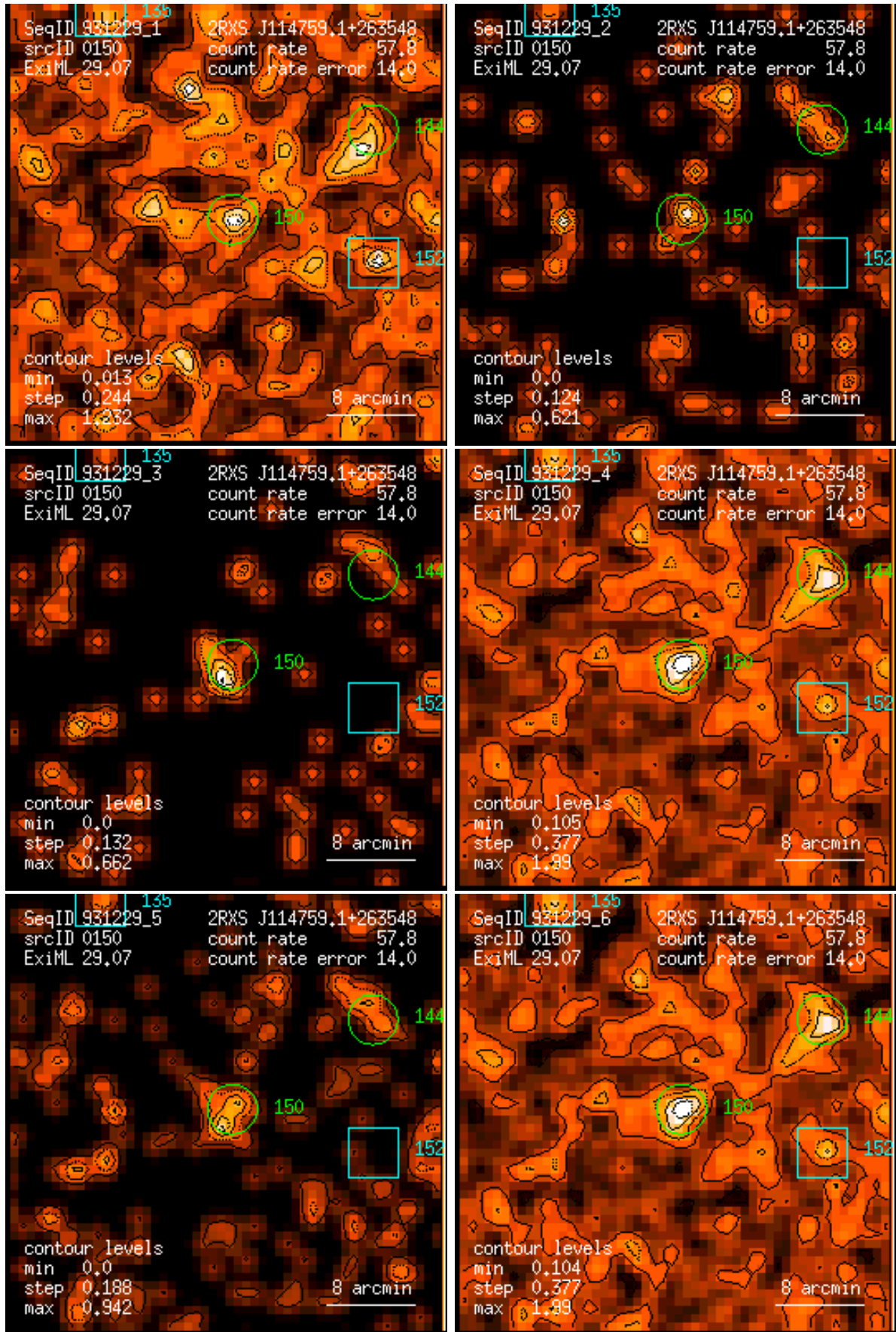
Figure 150: RASS 931229: detection 0150: band rate images, Gaussian filter: (1) PSPC channels 11 – 41, (2) 52 – 90, (3) 91 – 201, (4) 11 – 235, (5) 52 – 201, (6) 11 – 201. Broad band rates in counts/ks. Band rate contour levels in counts/ks/arcmin 2 .
