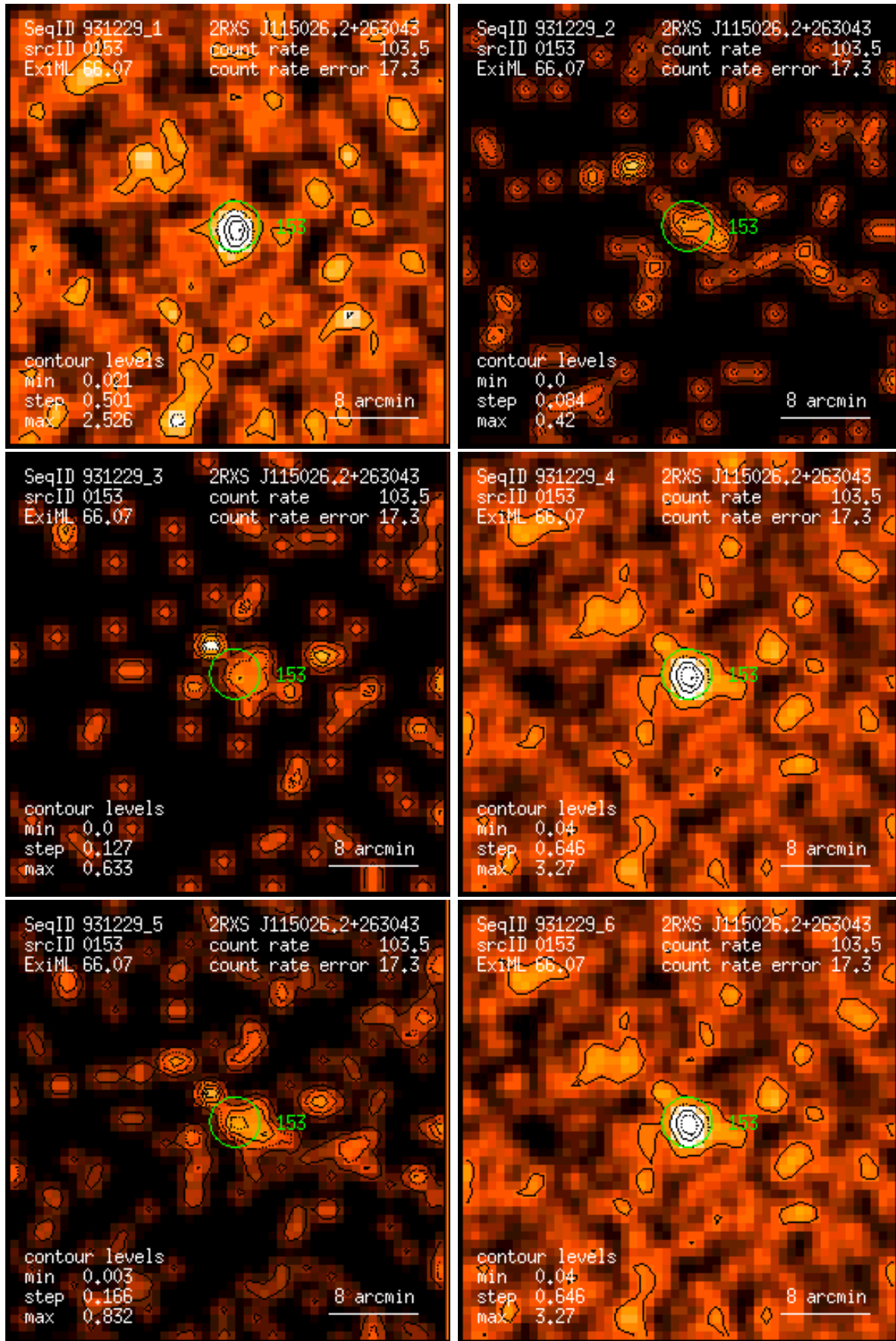
Figure 153: RASS 931229: detection 0153: band rate images, Gaussian filter: (1) PSPC channels 11 – 41, (2) 52 – 90, (3) 91 – 201, (4) 11 – 235, (5) 52 – 201, (6) 11 – 201. Broad band rates in counts/ks. Band rate contour levels in counts/ks/arcmin 2 .
