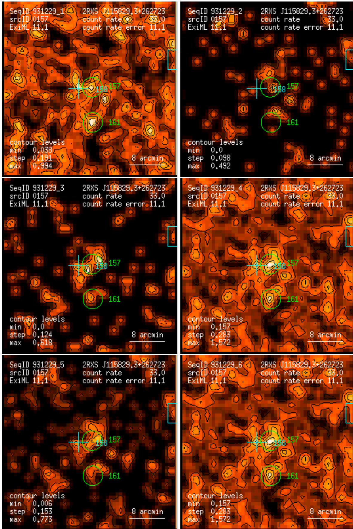
Figure 157: RASS 931229: detection 0157: band rate images, Gaussian filter: (1) PSPC channels 11 – 41, (2) 52 – 90, (3) 91 – 201, (4) 11 – 235, (5) 52 – 201, (6) 11 – 201. Broad band rates in counts/ks. Band rate contour levels in counts/ks/arcmin 2 .
