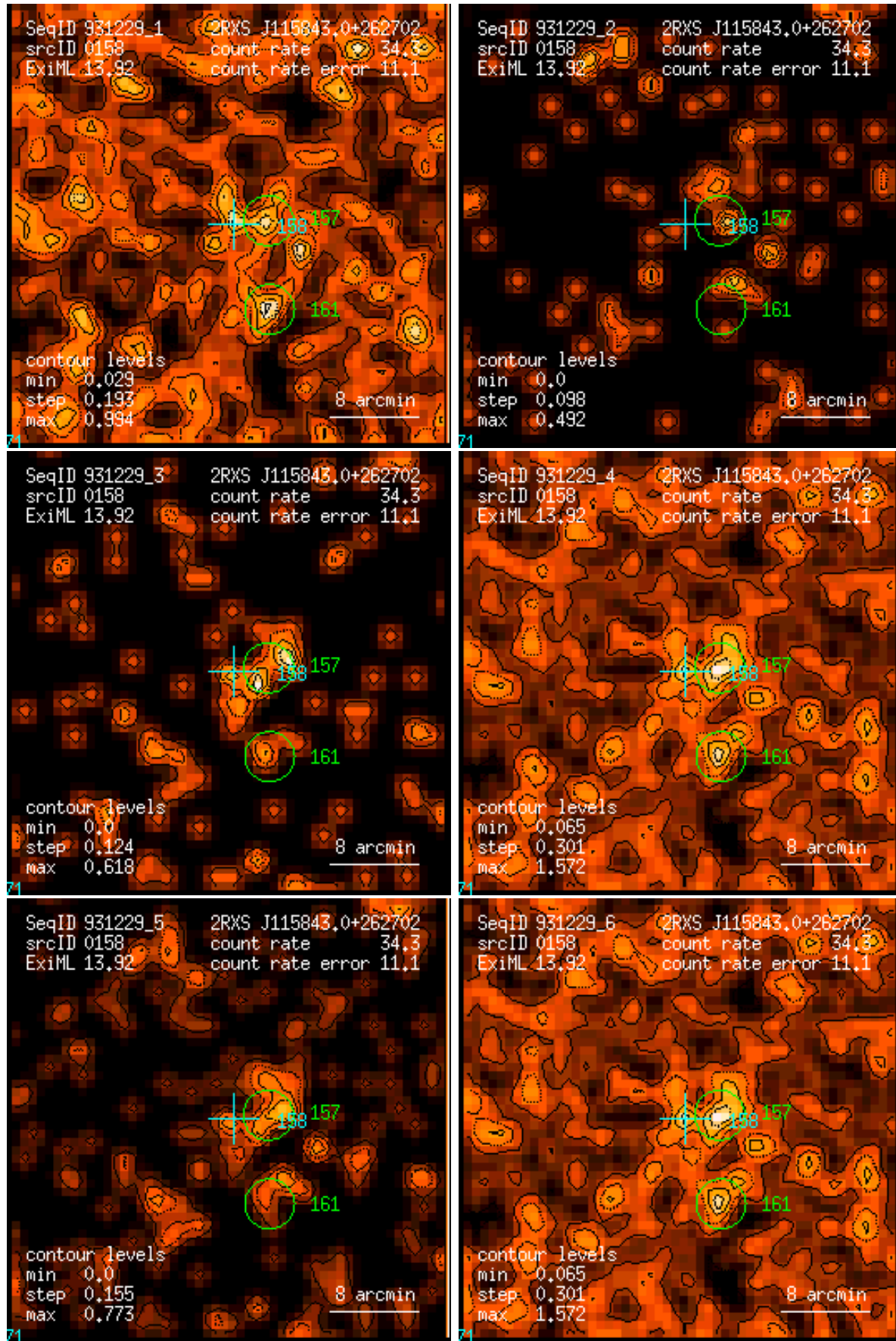
Figure 158: RASS 931229: detection 0158: band rate images, Gaussian filter: (1) PSPC channels 11 – 41, (2) 52 – 90, (3) 91 – 201, (4) 11 – 235, (5) 52 – 201, (6) 11 – 201. Broad band rates in counts/ks. Band rate contour levels in counts/ks/arcmin 2 .
