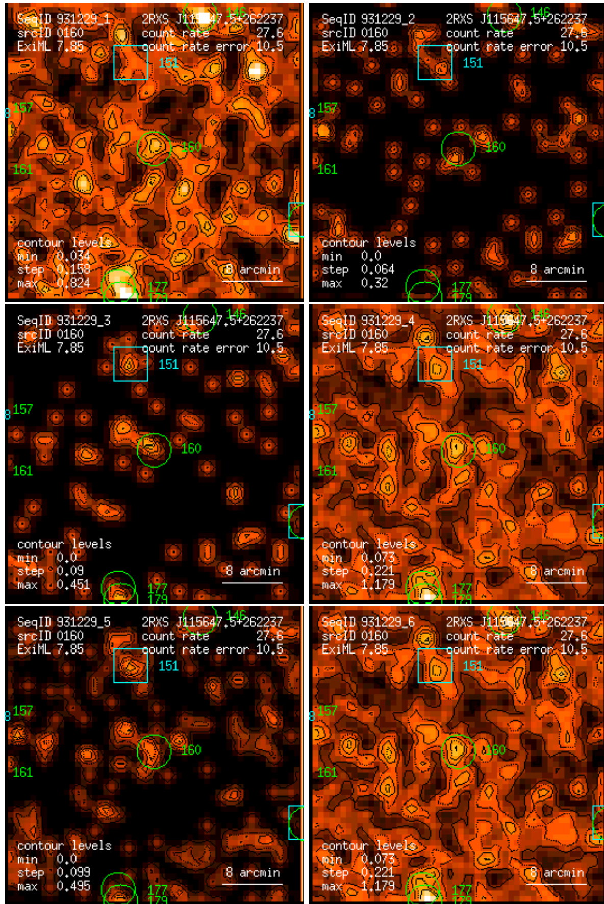
Figure 160: RASS 931229: detection 0160: band rate images, Gaussian filter: (1) PSPC channels 11 – 41, (2) 52 – 90, (3) 91 – 201, (4) 11 – 235, (5) 52 – 201, (6) 11 – 201. Broad band rates in counts/ks. Band rate contour levels in counts/ks/arcmin 2 .
