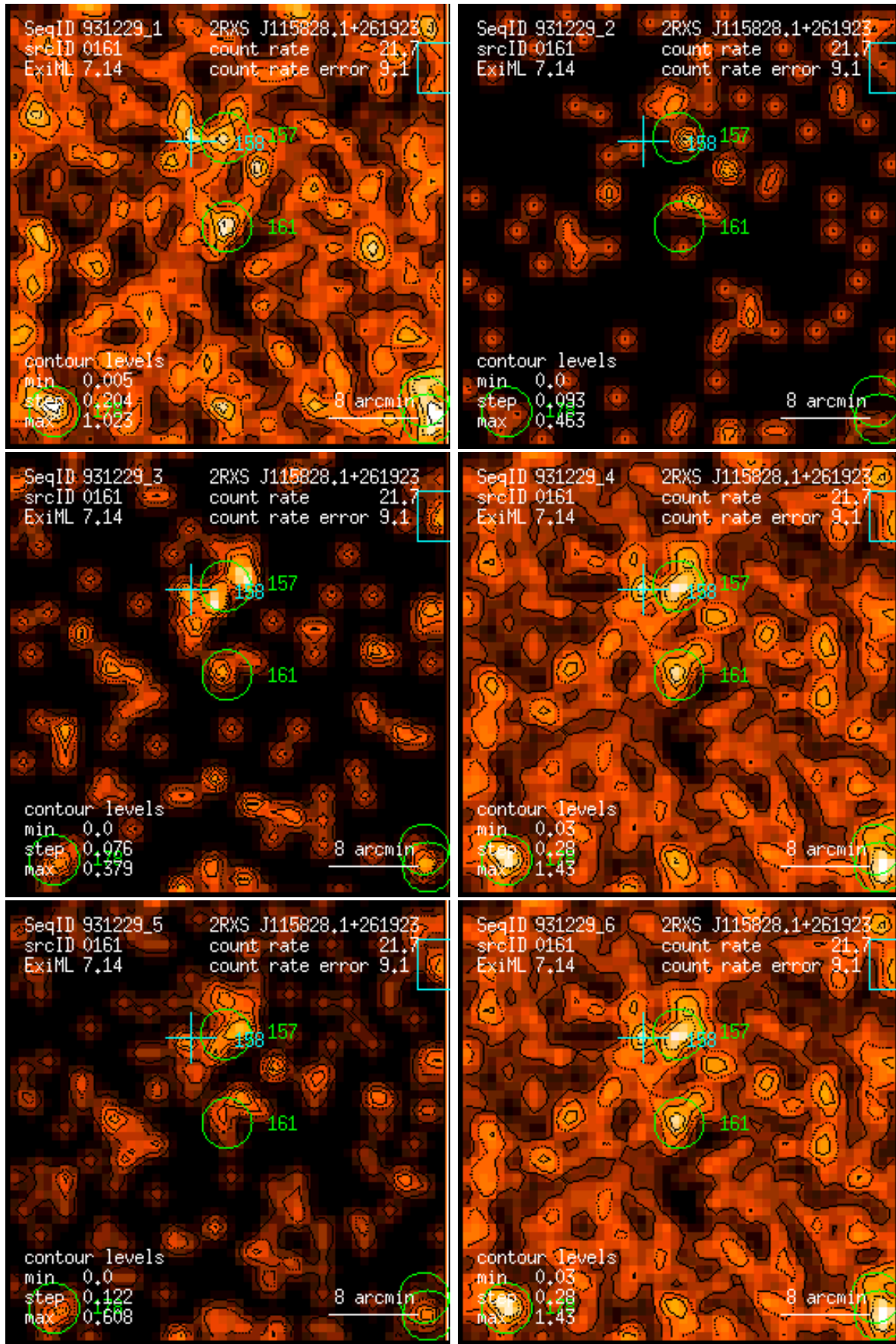
Figure 161: RASS 931229: detection 0161: band rate images, Gaussian filter: (1) PSPC channels 11 – 41, (2) 52 – 90, (3) 91 – 201, (4) 11 – 235, (5) 52 – 201, (6) 11 – 201. Broad band rates in counts/ks. Band rate contour levels in counts/ks/arcmin 2 .
