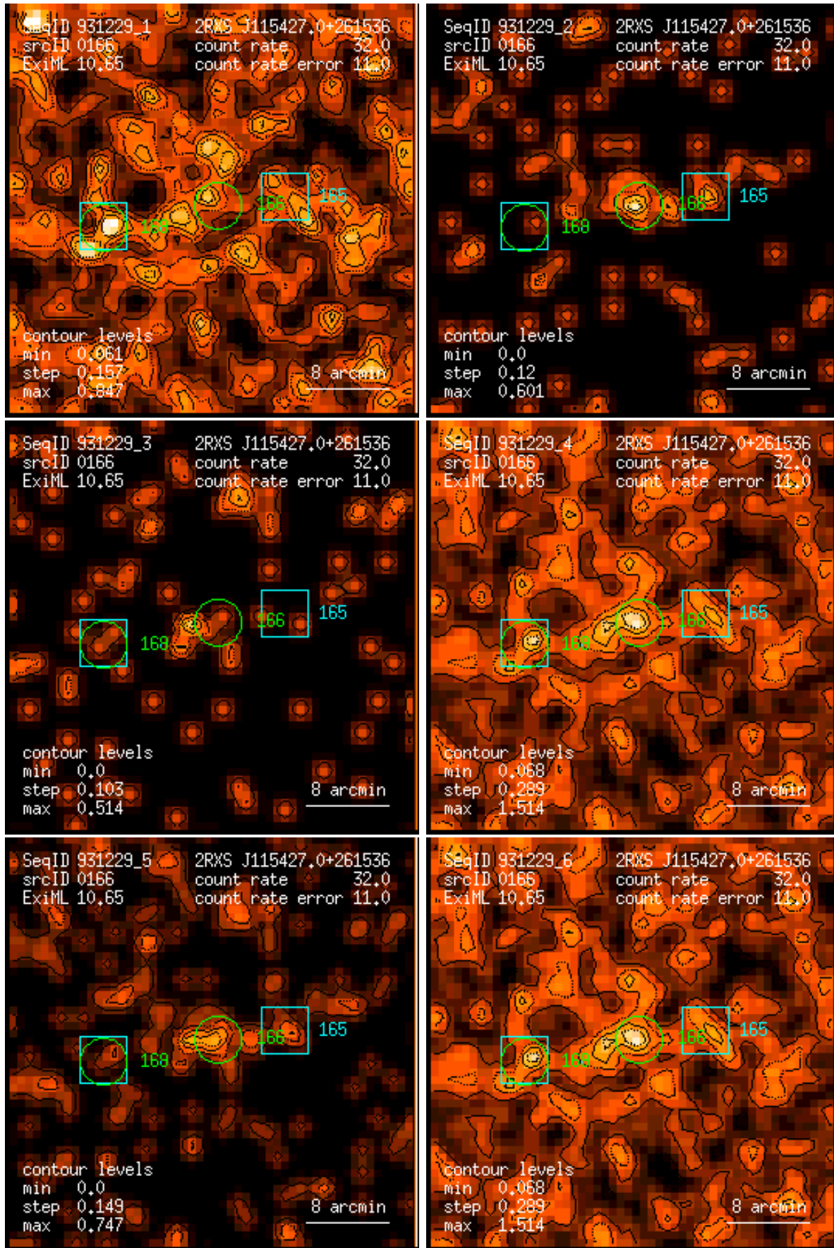
Figure 166: RASS 931229: detection 0166: band rate images, Gaussian filter: (1) PSPC channels 11 – 41, (2) 52 – 90, (3) 91 – 201, (4) 11 – 235, (5) 52 – 201, (6) 11 – 201. Broad band rates in counts/ks. Band rate contour levels in counts/ks/arcmin 2 .
