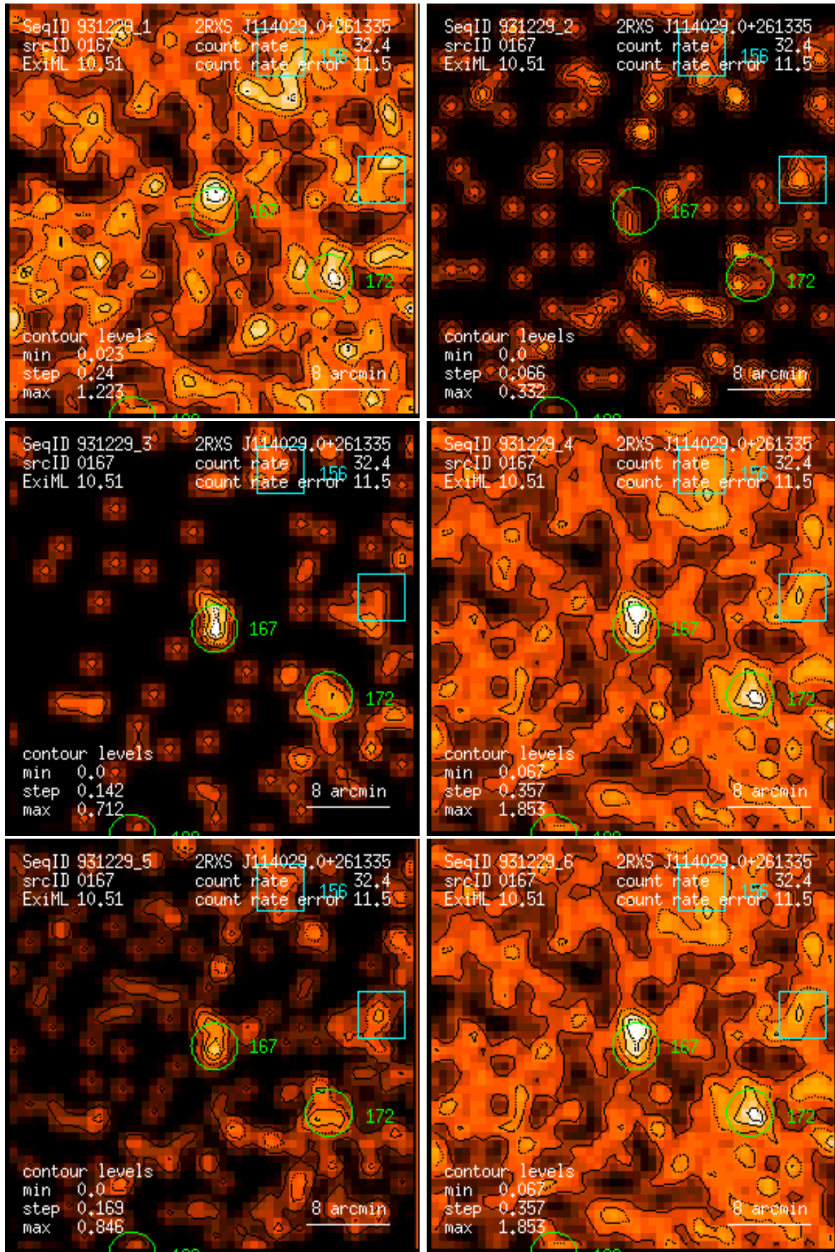
Figure 167: RASS 931229: detection 0167: band rate images, Gaussian filter: (1) PSPC channels 11 – 41, (2) 52 – 90, (3) 91 – 201, (4) 11 – 235, (5) 52 – 201, (6) 11 – 201. Broad band rates in counts/ks. Band rate contour levels in counts/ks/arcmin 2 .
