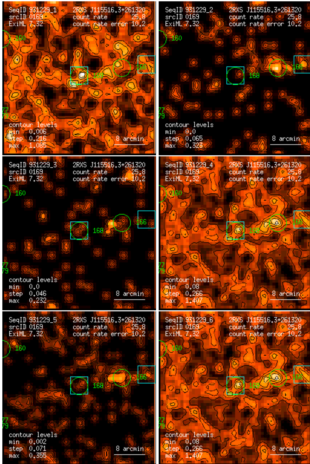
Figure 169: RASS 931229: detection 0169: band rate images, Gaussian filter: (1) PSPC channels 11 – 41, (2) 52 – 90, (3) 91 – 201, (4) 11 – 235, (5) 52 – 201, (6) 11 – 201. Broad band rates in counts/ks. Band rate contour levels in counts/ks/arcmin 2 .
