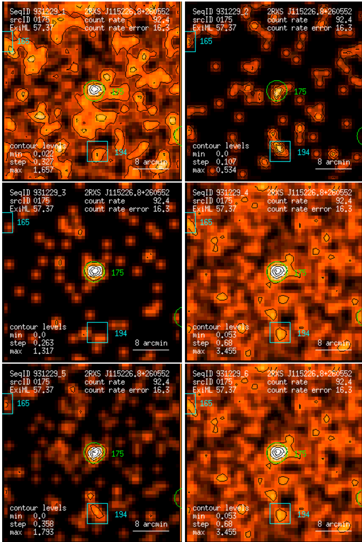
Figure 175: RASS 931229: detection 0175: band rate images, Gaussian filter: (1) PSPC channels 11 – 41, (2) 52 – 90, (3) 91 – 201, (4) 11 – 235, (5) 52 – 201, (6) 11 – 201. Broad band rates in counts/ks. Band rate contour levels in counts/ks/arcmin 2 .
