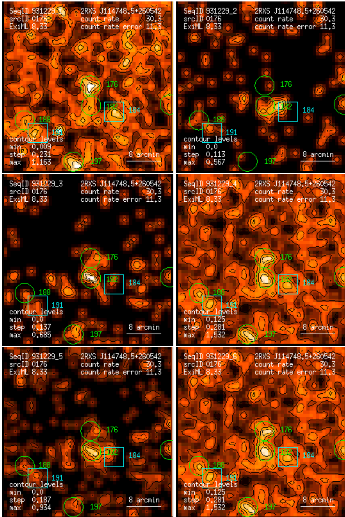
Figure 176: RASS 931229: detection 0176: band rate images, Gaussian filter: (1) PSPC channels 11 – 41, (2) 52 – 90, (3) 91 – 201, (4) 11 – 235, (5) 52 – 201, (6) 11 – 201. Broad band rates in counts/ks. Band rate contour levels in counts/ks/arcmin 2 .
