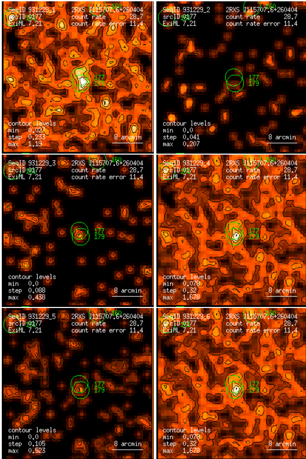
Figure 177: RASS 931229: detection 0177: band rate images, Gaussian filter: (1) PSPC channels 11 – 41, (2) 52 – 90, (3) 91 – 201, (4) 11 – 235, (5) 52 – 201, (6) 11 – 201. Broad band rates in counts/ks. Band rate contour levels in counts/ks/arcmin 2 .
