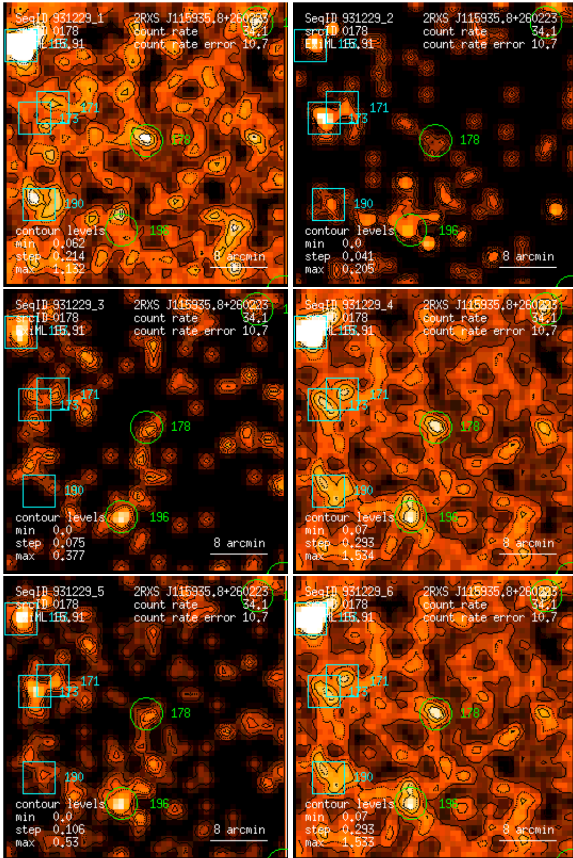
Figure 178: RASS 931229: detection 0178: band rate images, Gaussian filter: (1) PSPC channels 11 – 41, (2) 52 – 90, (3) 91 – 201, (4) 11 – 235, (5) 52 – 201, (6) 11 – 201. Broad band rates in counts/ks. Band rate contour levels in counts/ks/arcmin 2 .
