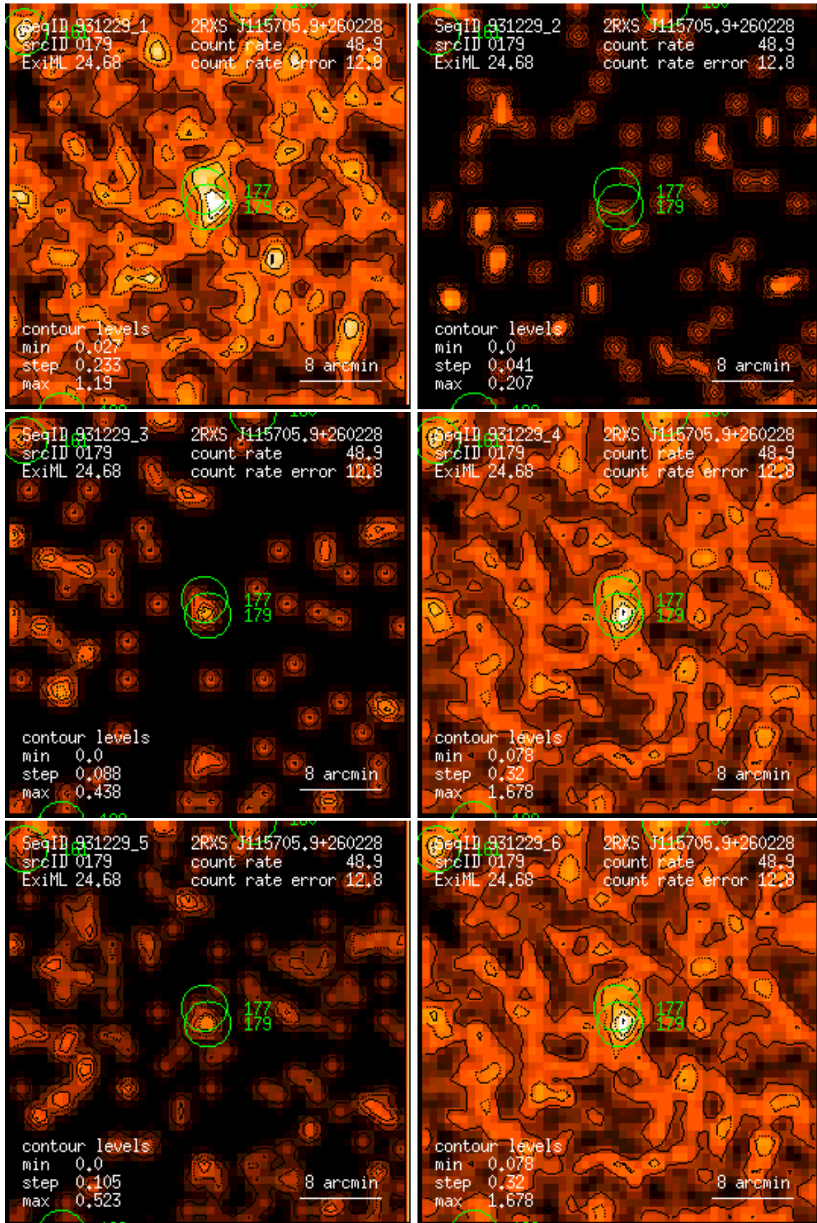
Figure 179: RASS 931229: detection 0179: band rate images, Gaussian filter: (1) PSPC channels 11 – 41, (2) 52 – 90, (3) 91 – 201, (4) 11 – 235, (5) 52 – 201, (6) 11 – 201. Broad band rates in counts/ks. Band rate contour levels in counts/ks/arcmin 2 .
