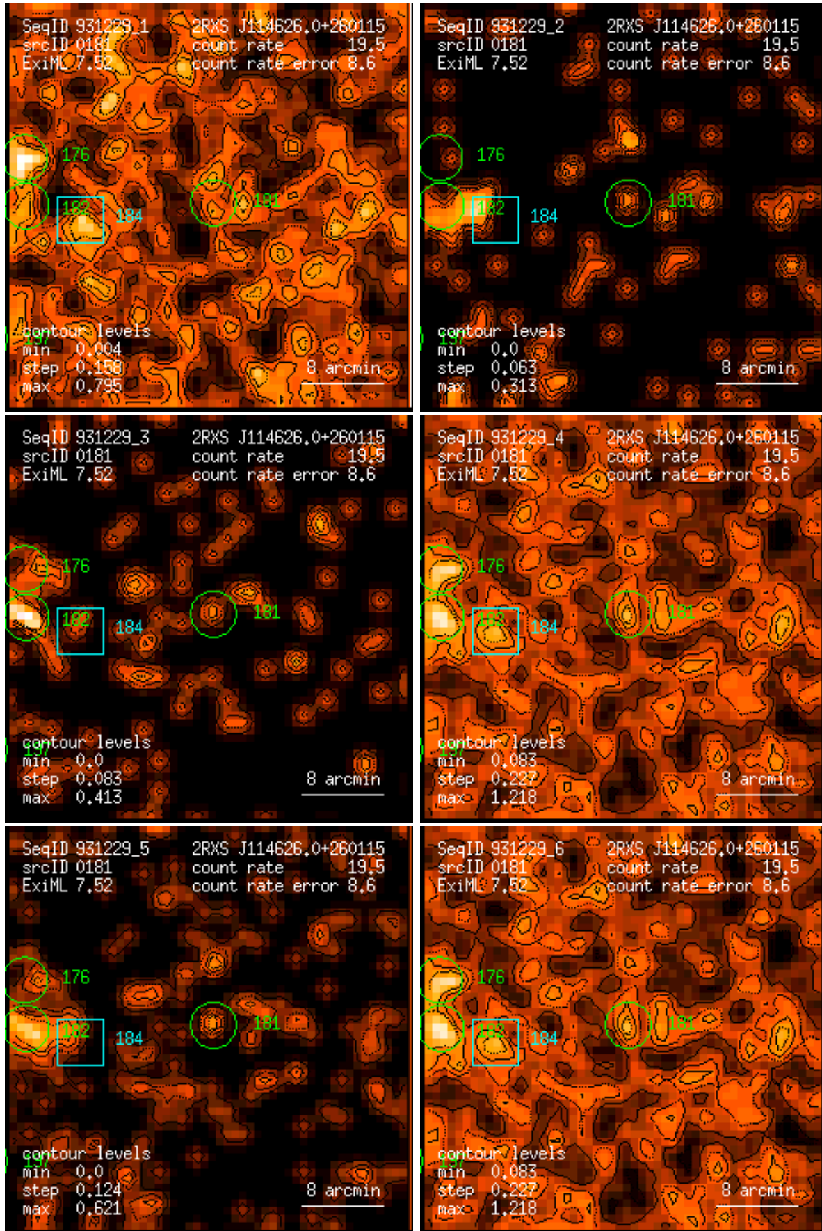
Figure 181: RASS 931229: detection 0181: band rate images, Gaussian filter: (1) PSPC channels 11 – 41, (2) 52 – 90, (3) 91 – 201, (4) 11 – 235, (5) 52 – 201, (6) 11 – 201. Broad band rates in counts/ks. Band rate contour levels in counts/ks/arcmin 2 .
