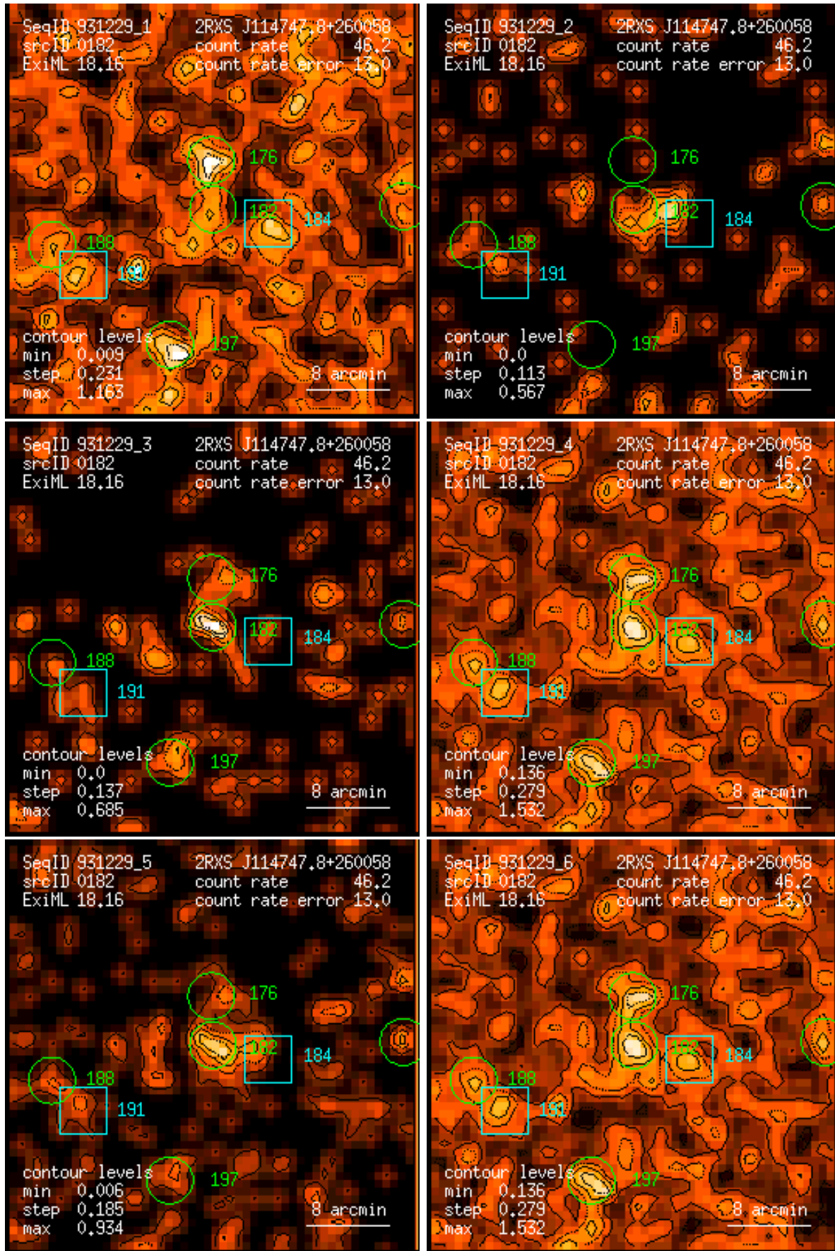
Figure 182: RASS 931229: detection 0182: band rate images, Gaussian filter: (1) PSPC channels 11 – 41, (2) 52 – 90, (3) 91 – 201, (4) 11 – 235, (5) 52 – 201, (6) 11 – 201. Broad band rates in counts/ks. Band rate contour levels in counts/ks/arcmin 2 .
