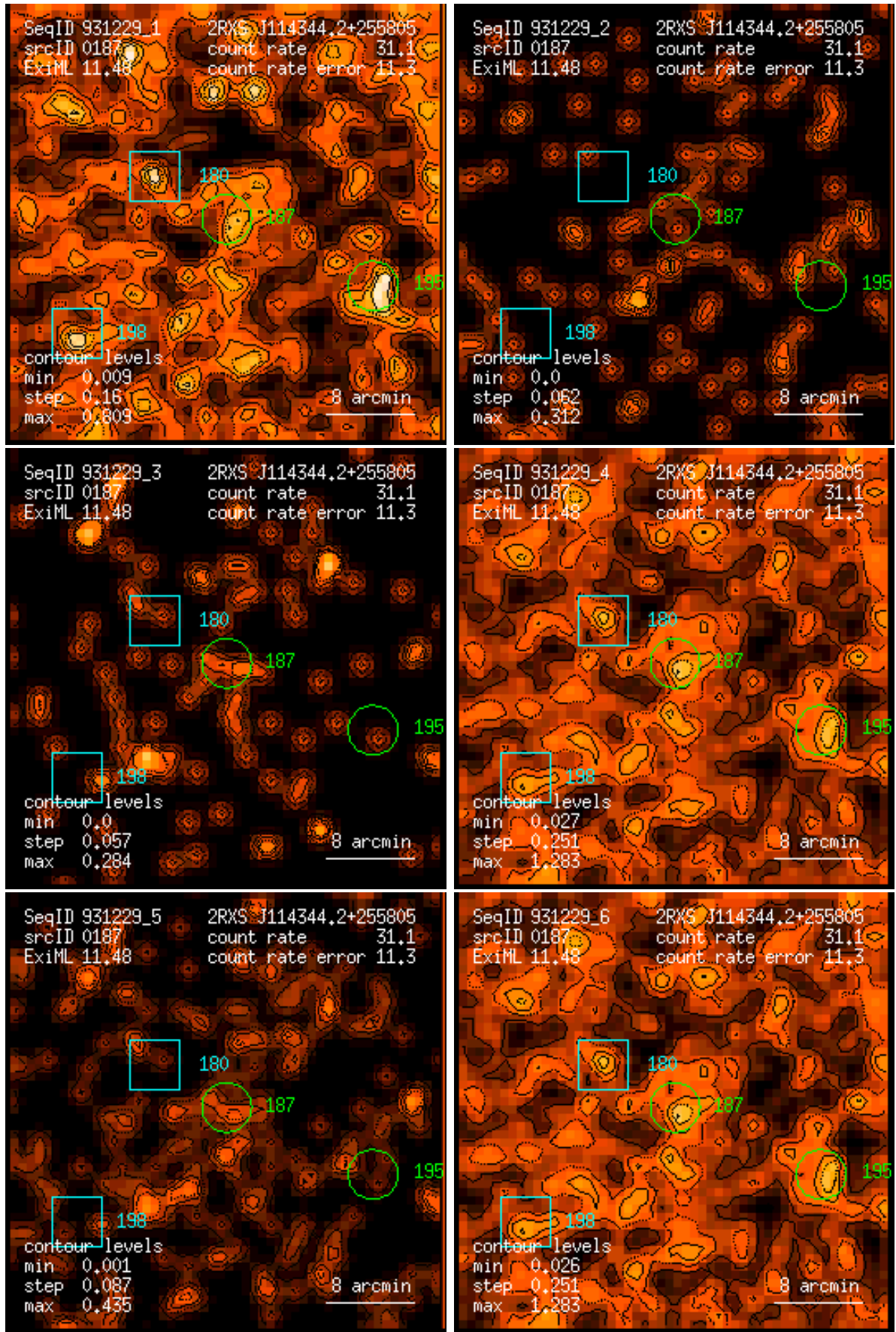
Figure 187: RASS 931229: detection 0187: band rate images, Gaussian filter: (1) PSPC channels 11 – 41, (2) 52 – 90, (3) 91 – 201, (4) 11 – 235, (5) 52 – 201, (6) 11 – 201. Broad band rates in counts/ks. Band rate contour levels in counts/ks/arcmin 2 .
