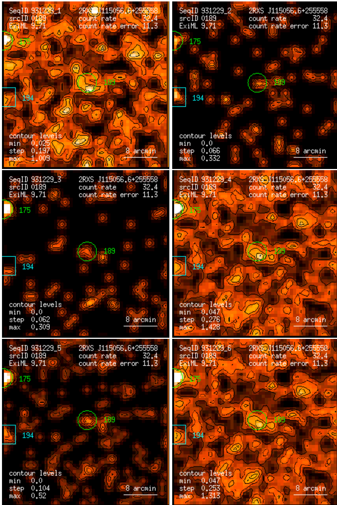
Figure 189: RASS 931229: detection 0189: band rate images, Gaussian filter: (1) PSPC channels 11 – 41, (2) 52 – 90, (3) 91 – 201, (4) 11 – 235, (5) 52 – 201, (6) 11 – 201. Broad band rates in counts/ks. Band rate contour levels in counts/ks/arcmin 2 .
