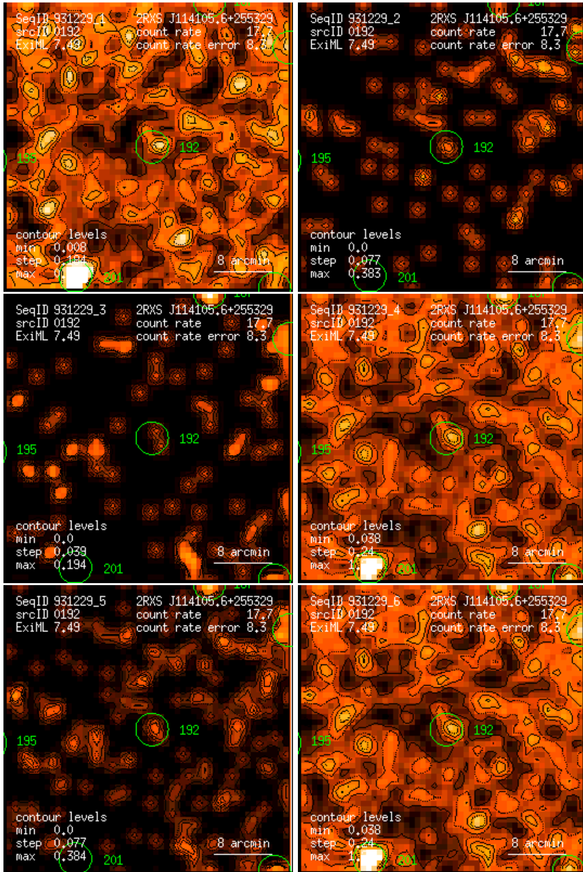
Figure 192: RASS 931229: detection 0192: band rate images, Gaussian filter: (1) PSPC channels 11 – 41, (2) 52 – 90, (3) 91 – 201, (4) 11 – 235, (5) 52 – 201, (6) 11 – 201. Broad band rates in counts/ks. Band rate contour levels in counts/ks/arcmin 2 .
